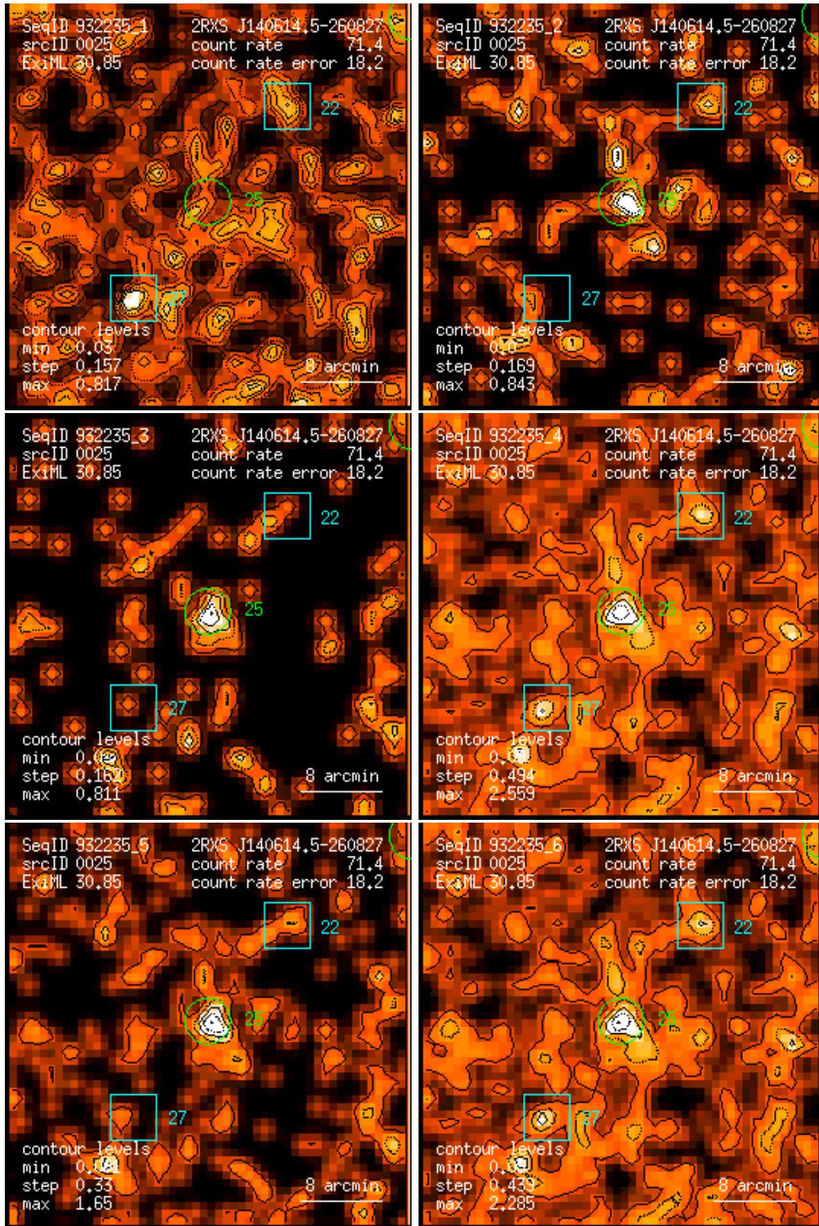
Figure 25: RASS 932235: detection 0025: band rate images, Gaussian filter: (1) PSPC channels 11 – 41, (2) 52 – 90, (3) 91 – 201, (4) 11 – 235, (5) 52 – 201, (6) 11 – 201. Broad band rates in counts/ks. Band rate contour levels in counts/ks/arcmin 2 .
