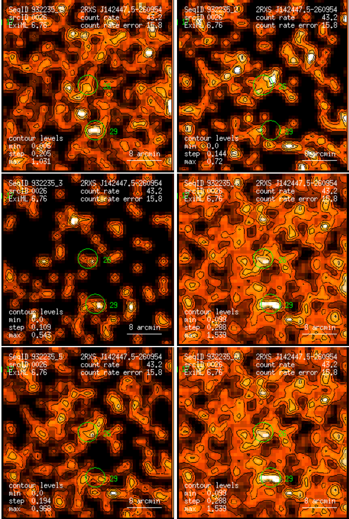
Figure 26: RASS 932235: detection 0026: band rate images, Gaussian filter: (1) PSPC channels 11 – 41, (2) 52 – 90, (3) 91 – 201, (4) 11 – 235, (5) 52 – 201, (6) 11 – 201. Broad band rates in counts/ks. Band rate contour levels in counts/ks/arcmin 2 .
