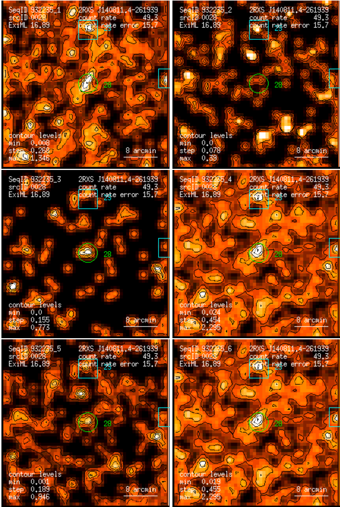
Figure 28: RASS 932235: detection 0028: band rate images, Gaussian filter: (1) PSPC channels 11 – 41, (2) 52 – 90, (3) 91 – 201, (4) 11 – 235, (5) 52 – 201, (6) 11 – 201. Broad band rates in counts/ks. Band rate contour levels in counts/ks/arcmin 2 .
