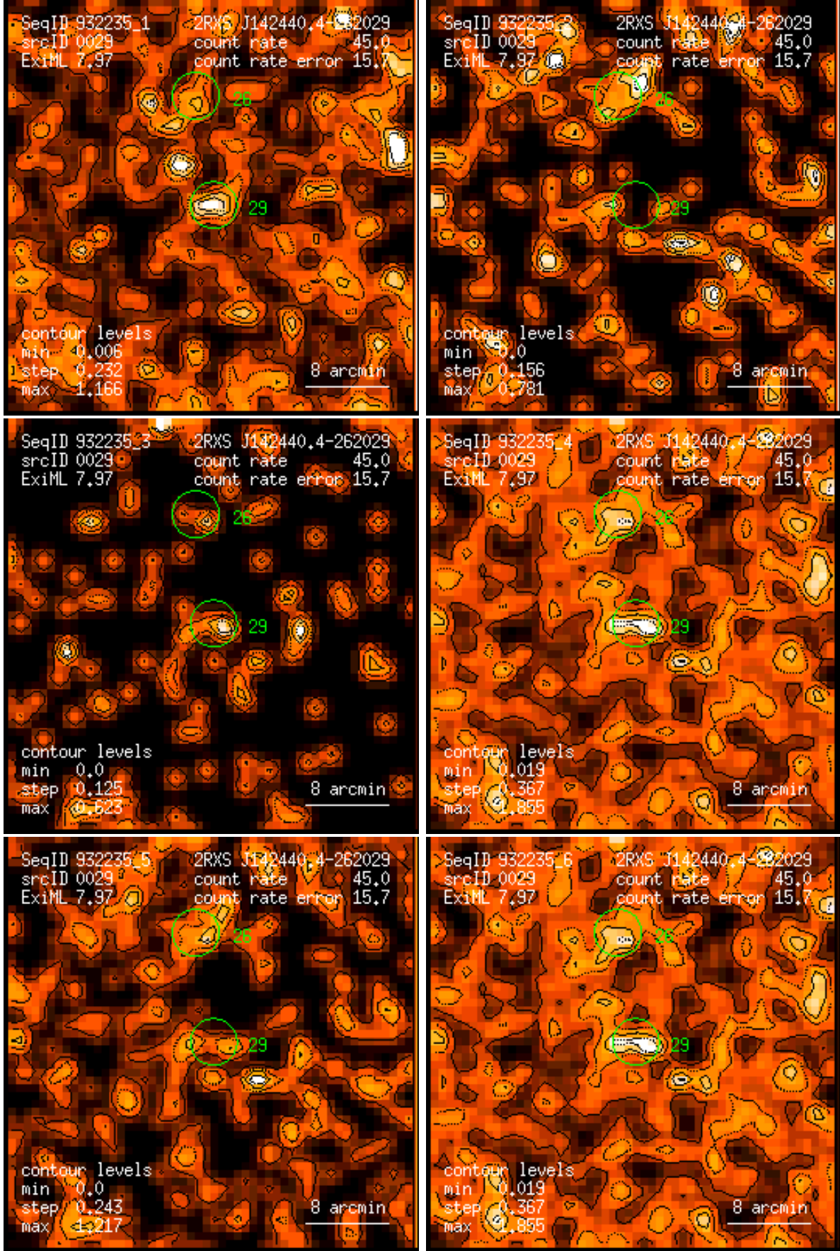
Figure 29: RASS 932235: detection 0029: band rate images, Gaussian filter: (1) PSPC channels 11 – 41, (2) 52 – 90, (3) 91 – 201, (4) 11 – 235, (5) 52 – 201, (6) 11 – 201. Broad band rates in counts/ks. Band rate contour levels in counts/ks/arcmin 2 .
