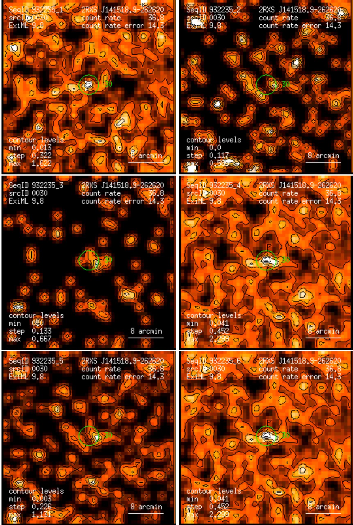
Figure 30: RASS 932235: detection 0030: band rate images, Gaussian filter: (1) PSPC channels 11 – 41, (2) 52 – 90, (3) 91 – 201, (4) 11 – 235, (5) 52 – 201, (6) 11 – 201. Broad band rates in counts/ks. Band rate contour levels in counts/ks/arcmin 2 .
