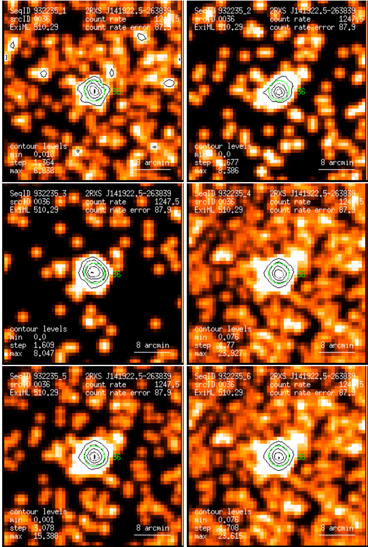
Figure 36: RASS 932235: detection 0036: band rate images, Gaussian filter: (1) PSPC channels 11 – 41, (2) 52 – 90, (3) 91 – 201, (4) 11 – 235, (5) 52 – 201, (6) 11 – 201. Broad band rates in counts/ks. Band rate contour levels in counts/ks/arcmin 2 .
