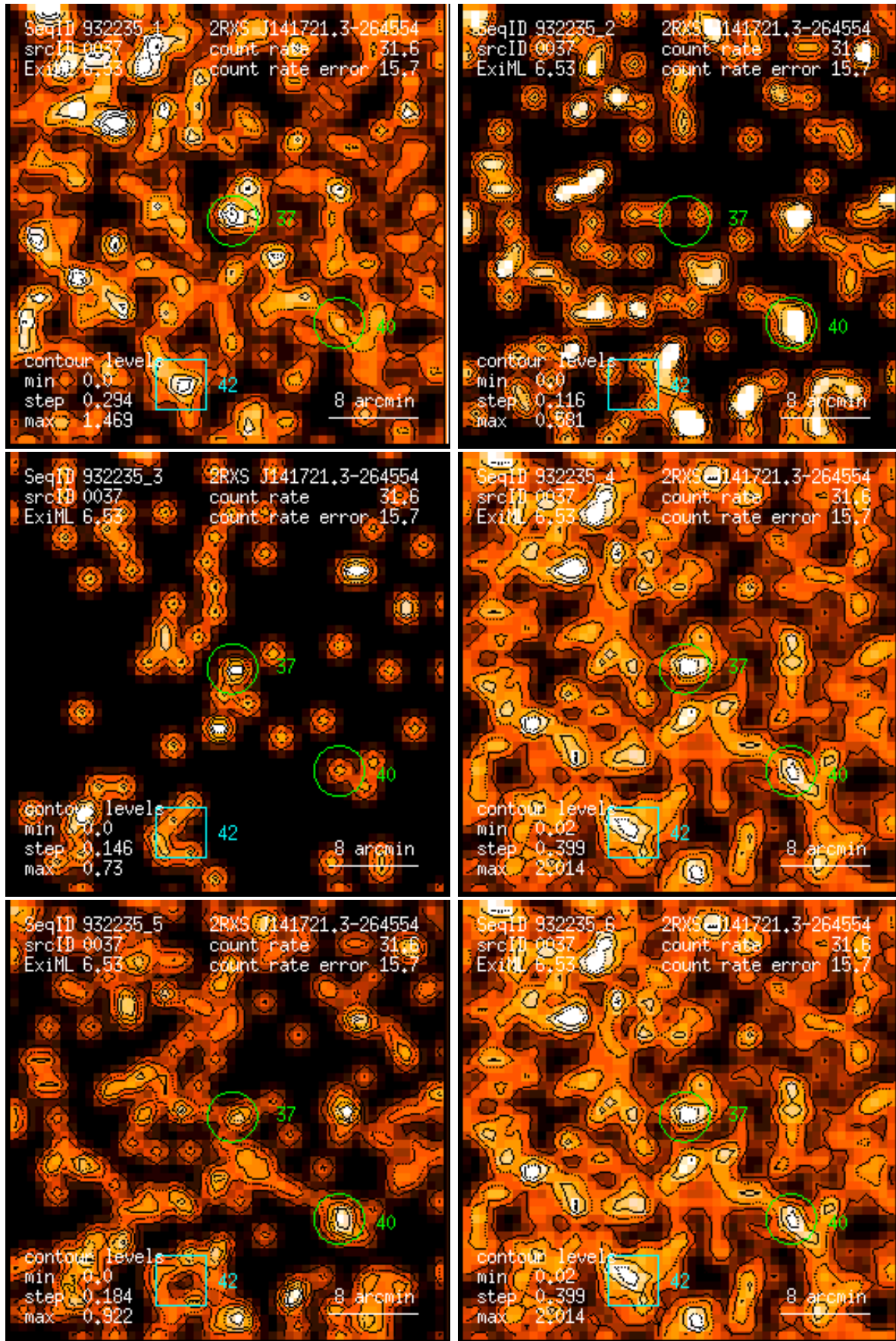
Figure 37: RASS 932235: detection 0037: band rate images, Gaussian filter: (1) PSPC channels 11 – 41, (2) 52 – 90, (3) 91 – 201, (4) 11 – 235, (5) 52 – 201, (6) 11 – 201. Broad band rates in counts/ks. Band rate contour levels in counts/ks/arcmin 2 .
