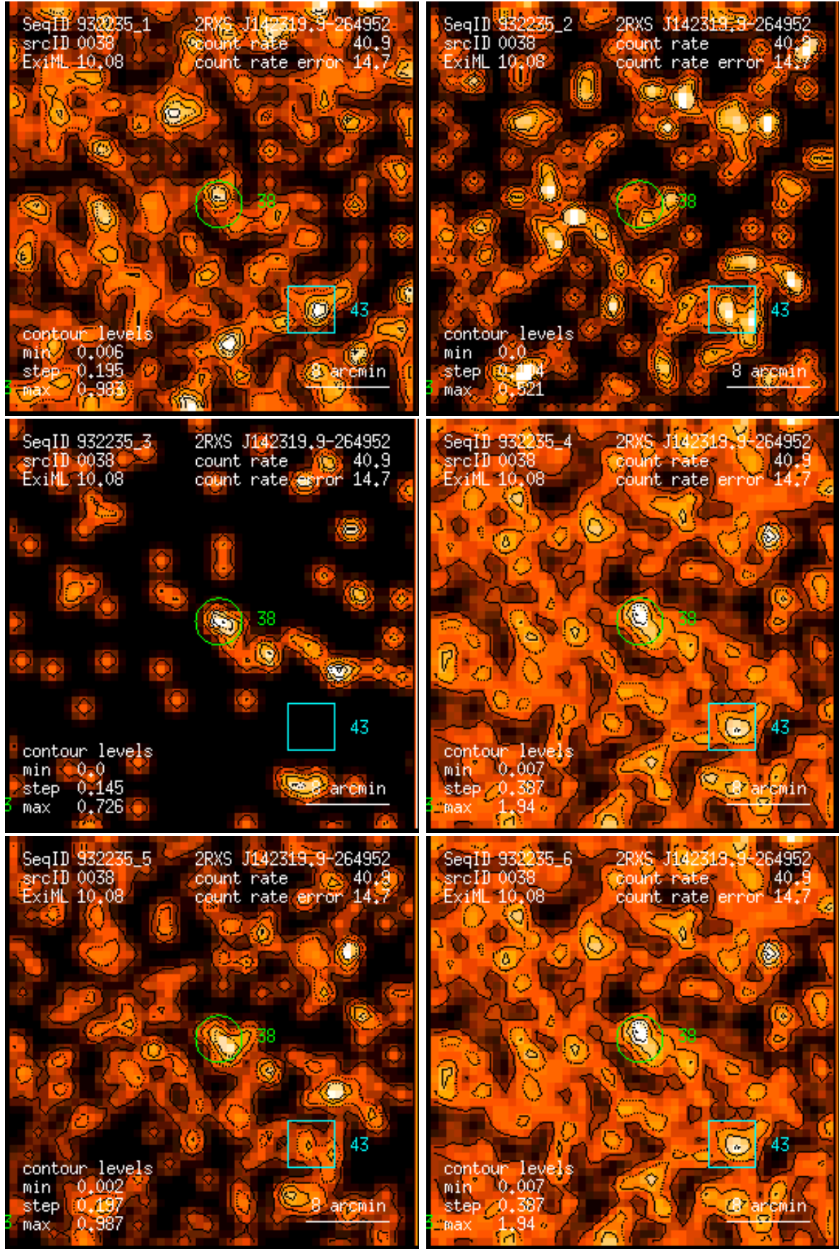
Figure 38: RASS 932235: detection 0038: band rate images, Gaussian filter: (1) PSPC channels 11 – 41, (2) 52 – 90, (3) 91 – 201, (4) 11 – 235, (5) 52 – 201, (6) 11 – 201. Broad band rates in counts/ks. Band rate contour levels in counts/ks/arcmin 2 .
