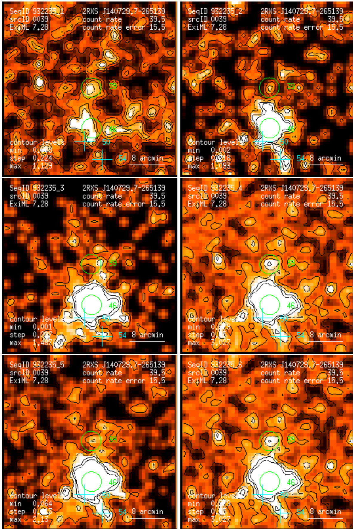
Figure 39: RASS 932235: detection 0039: band rate images, Gaussian filter: (1) PSPC channels 11 – 41, (2) 52 – 90, (3) 91 – 201, (4) 11 – 235, (5) 52 – 201, (6) 11 – 201. Broad band rates in counts/ks. Band rate contour levels in counts/ks/arcmin 2 .
