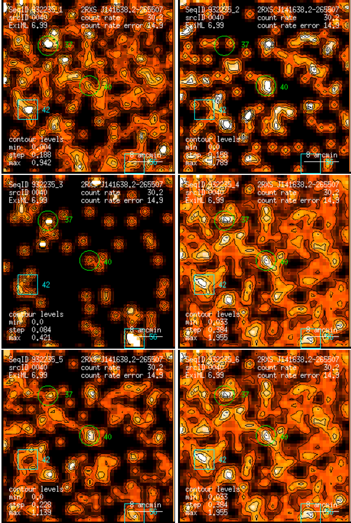
Figure 40: RASS 932235: detection 0040: band rate images, Gaussian filter: (1) PSPC channels 11 – 41, (2) 52 – 90, (3) 91 – 201, (4) 11 – 235, (5) 52 – 201, (6) 11 – 201. Broad band rates in counts/ks. Band rate contour levels in counts/ks/arcmin 2 .
