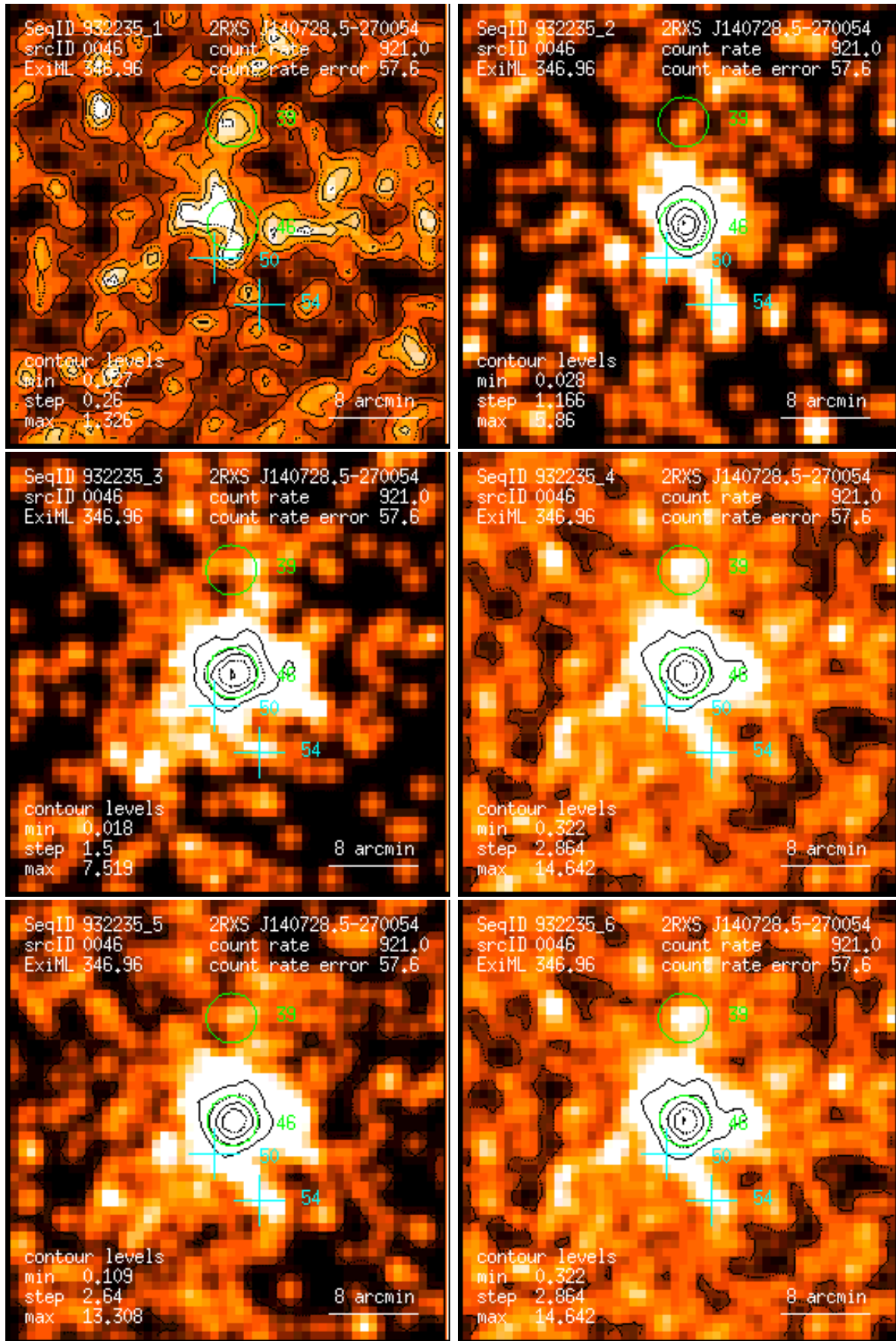
Figure 46: RASS 932235: detection 0046: band rate images, Gaussian filter: (1) PSPC channels 11 – 41, (2) 52 – 90, (3) 91 – 201, (4) 11 – 235, (5) 52 – 201, (6) 11 – 201. Broad band rates in counts/ks. Band rate contour levels in counts/ks/arcmin 2 .
