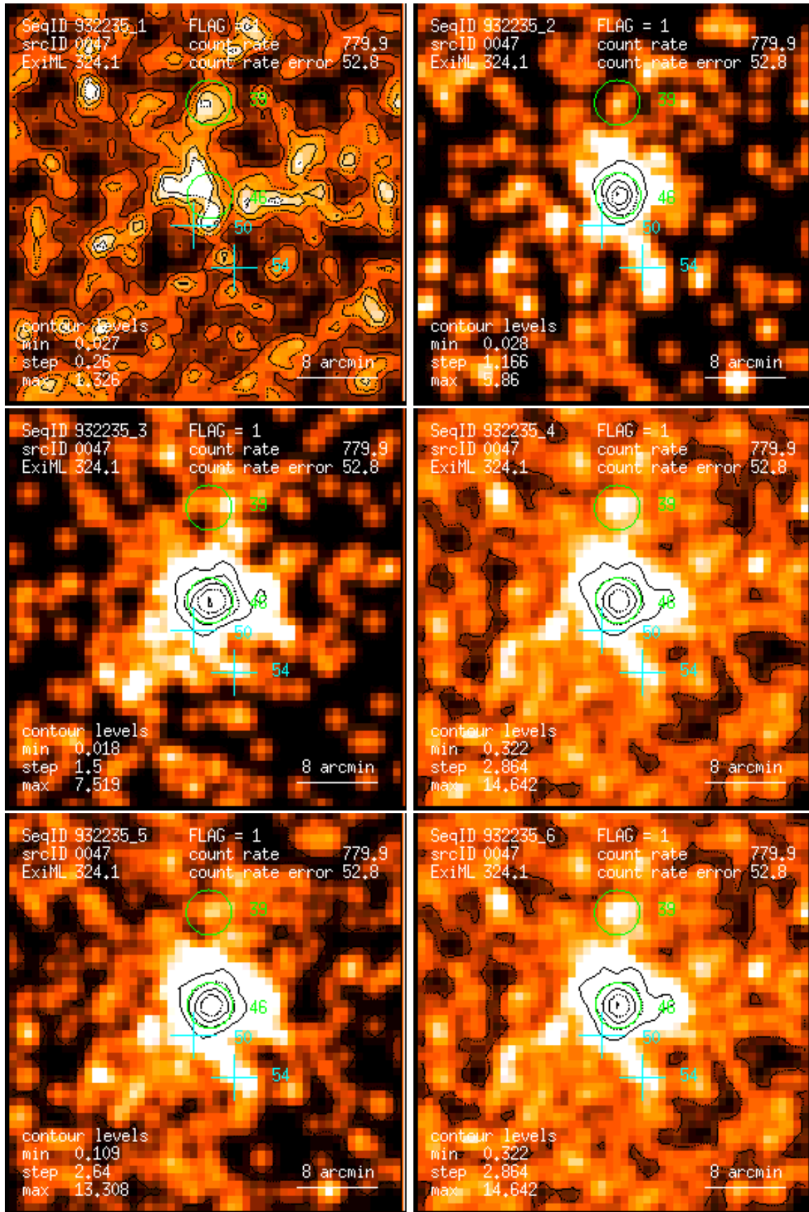
Figure 47: RASS 932235: detection 0047: band rate images, Gaussian filter: (1) PSPC channels 11 – 41, (2) 52 – 90, (3) 91 – 201, (4) 11 – 235, (5) 52 – 201, (6) 11 – 201. Broad band rates in counts/ks. Band rate contour levels in counts/ks/arcmin 2 .
