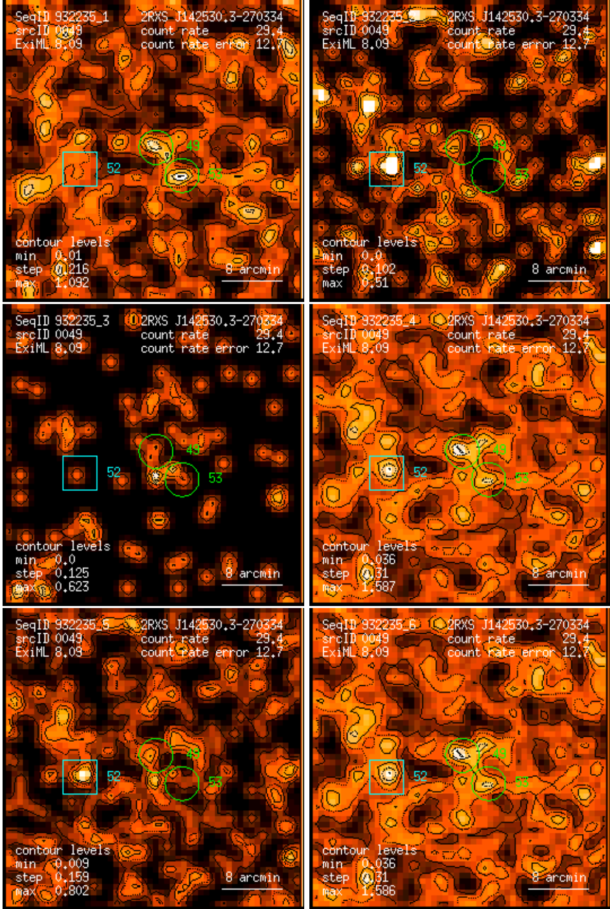
Figure 49: RASS 932235: detection 0049: band rate images, Gaussian filter: (1) PSPC channels 11 – 41, (2) 52 – 90, (3) 91 – 201, (4) 11 – 235, (5) 52 – 201, (6) 11 – 201. Broad band rates in counts/ks. Band rate contour levels in counts/ks/arcmin 2 .
