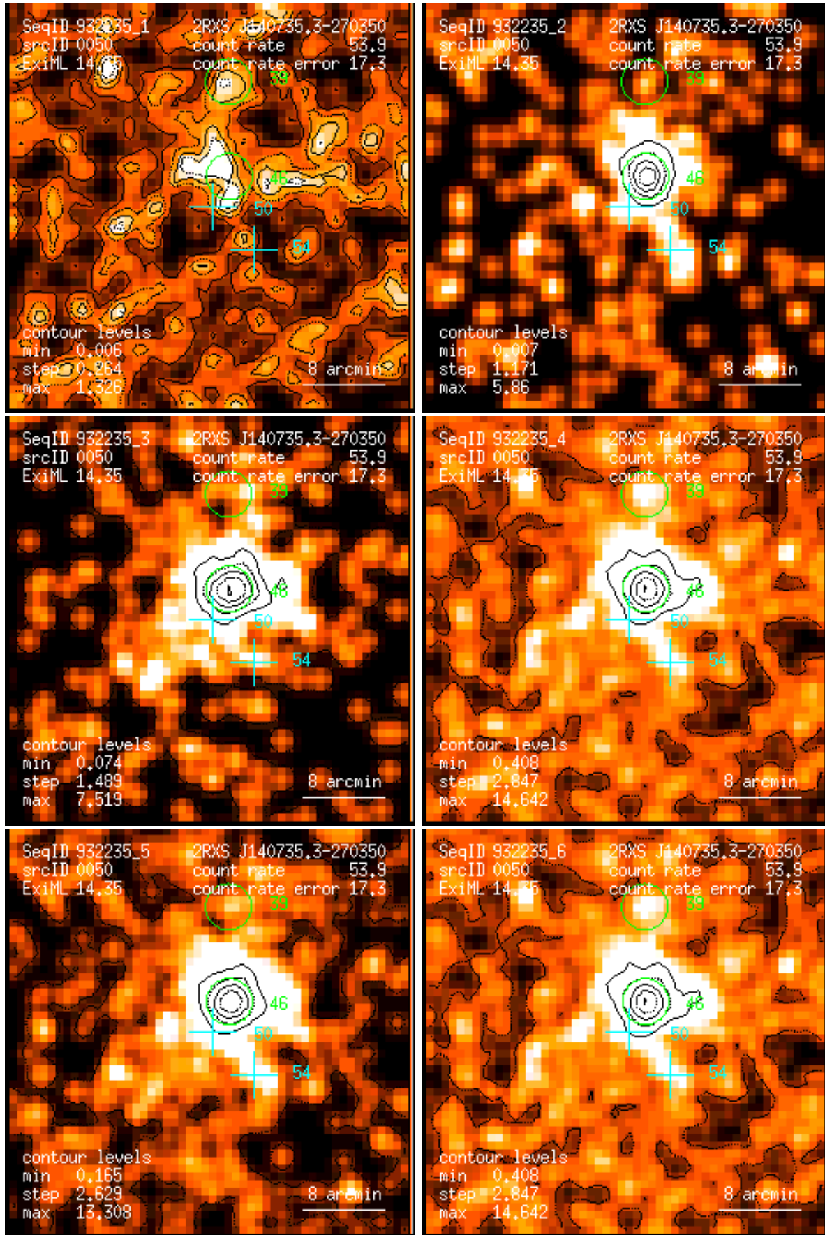
Figure 50: RASS 932235: detection 0050: band rate images, Gaussian filter: (1) PSPC channels 11 – 41, (2) 52 – 90, (3) 91 – 201, (4) 11 – 235, (5) 52 – 201, (6) 11 – 201. Broad band rates in counts/ks. Band rate contour levels in counts/ks/arcmin 2 .
