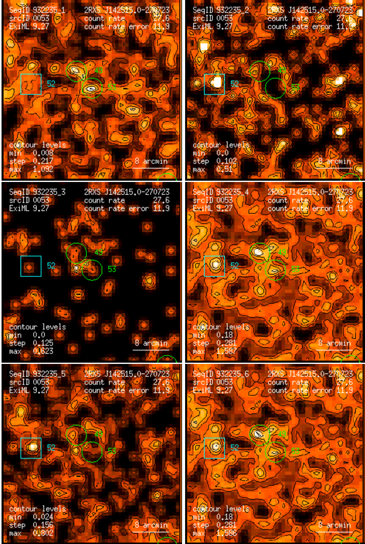
Figure 53: RASS 932235: detection 0053: band rate images, Gaussian filter: (1) PSPC channels 11 – 41, (2) 52 – 90, (3) 91 – 201, (4) 11 – 235, (5) 52 – 201, (6) 11 – 201. Broad band rates in counts/ks. Band rate contour levels in counts/ks/arcmin 2 .
