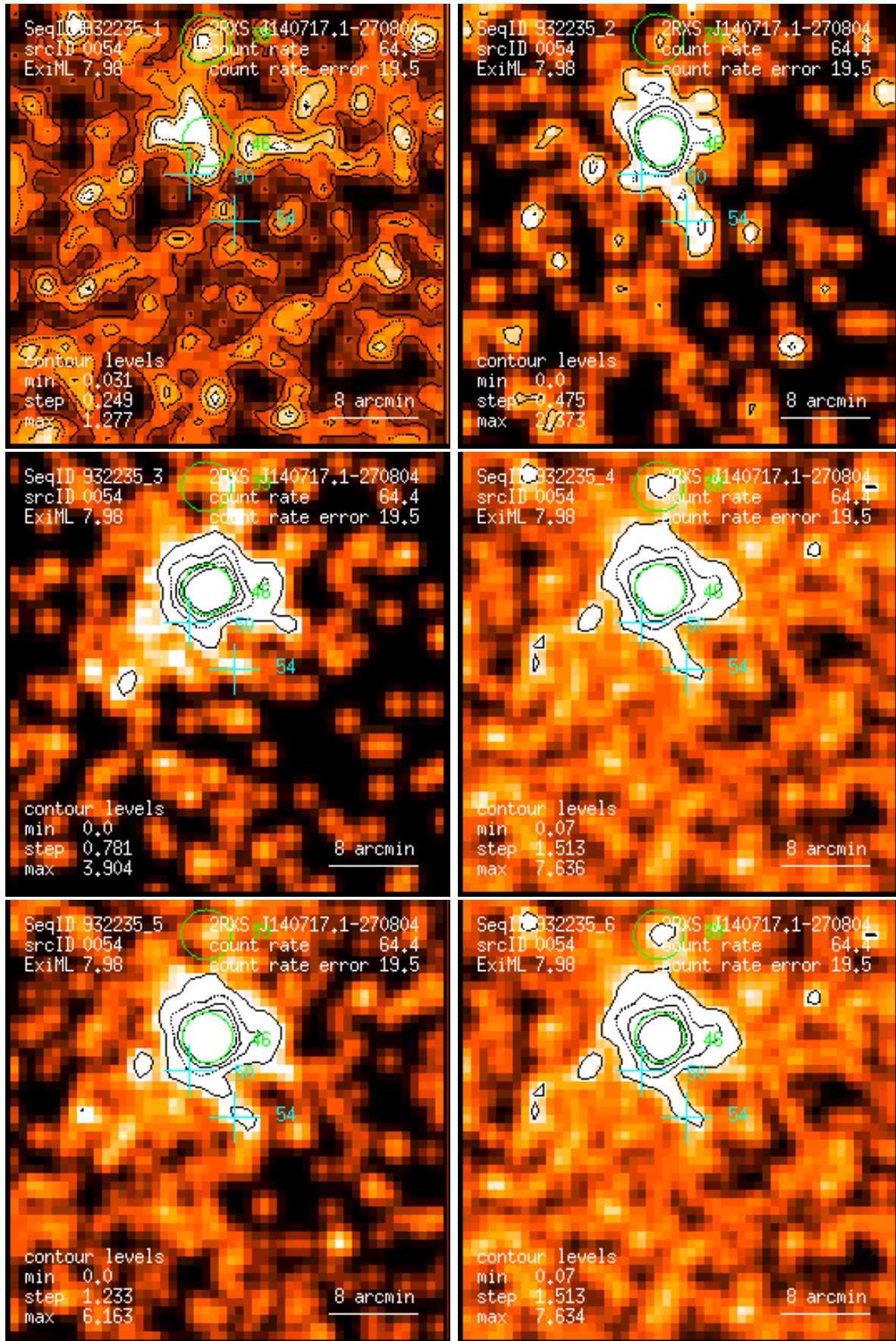
Figure 54: RASS 932235: detection 0054: band rate images, Gaussian filter: (1) PSPC channels 11 – 41, (2) 52 – 90, (3) 91 – 201, (4) 11 – 235, (5) 52 – 201, (6) 11 – 201. Broad band rates in counts/ks. Band rate contour levels in counts/ks/arcmin 2 .
