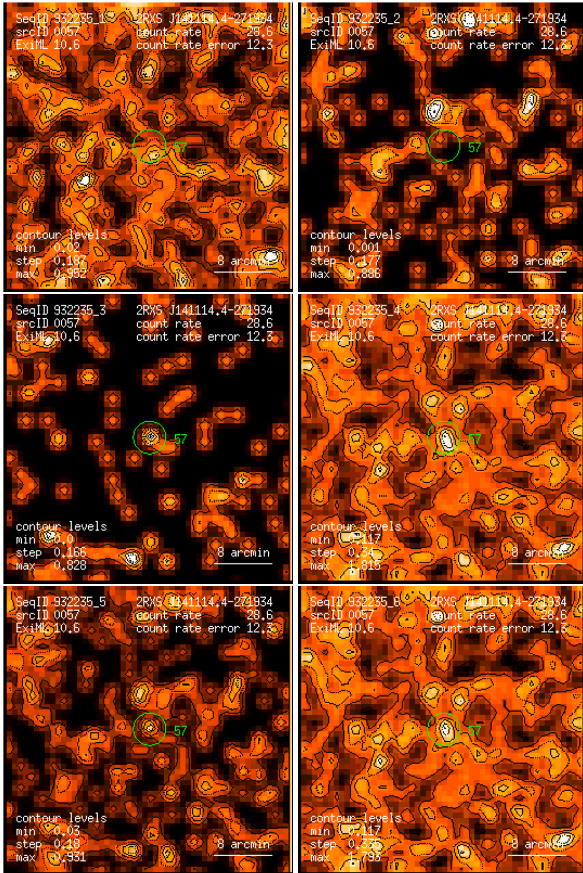
Figure 57: RASS 932235: detection 0057: band rate images, Gaussian filter: (1) PSPC channels 11 – 41, (2) 52 – 90, (3) 91 – 201, (4) 11 – 235, (5) 52 – 201, (6) 11 – 201. Broad band rates in counts/ks. Band rate contour levels in counts/ks/arcmin 2 .
