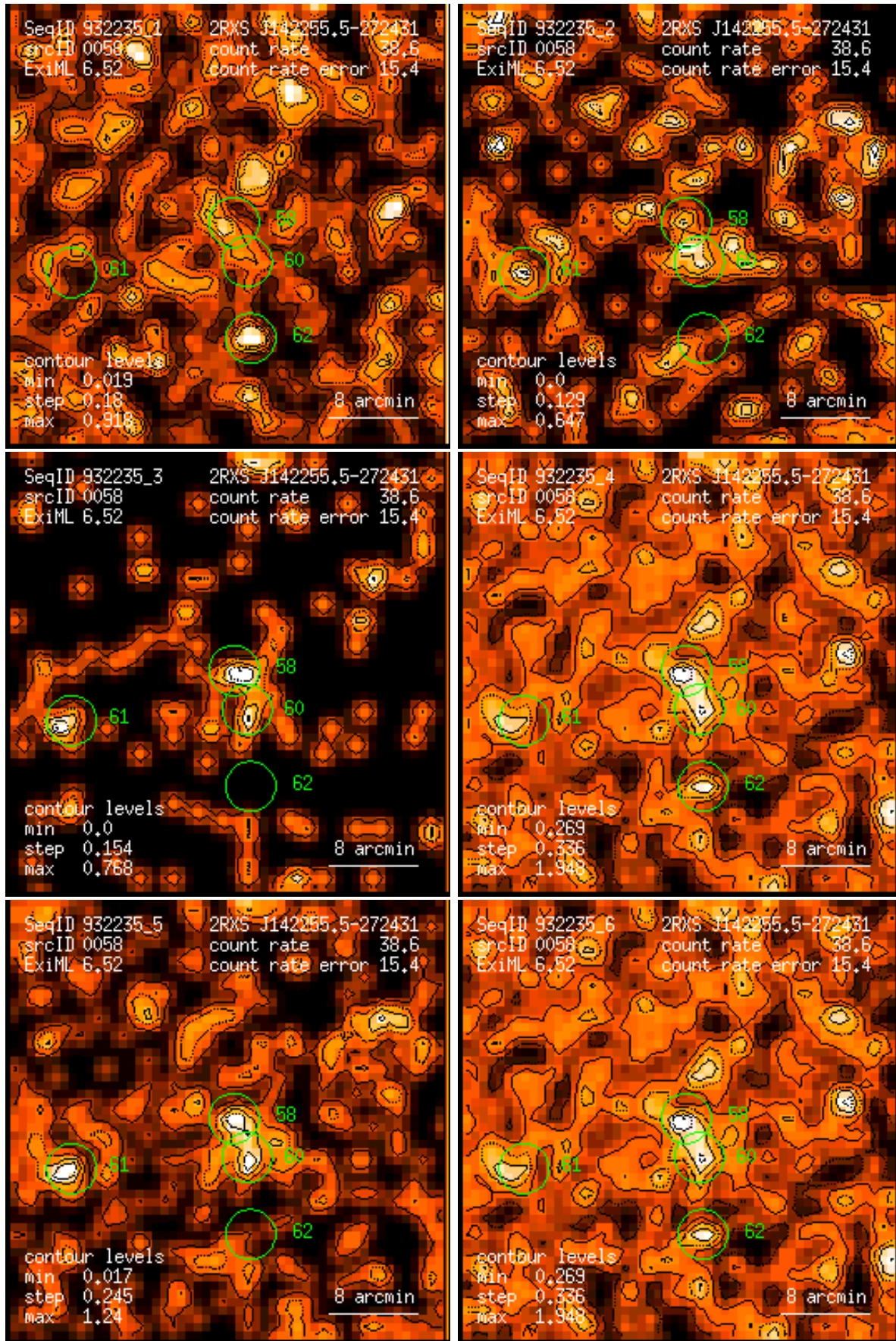
Figure 58: RASS 932235: detection 0058: band rate images, Gaussian filter: (1) PSPC channels 11 – 41, (2) 52 – 90, (3) 91 – 201, (4) 11 – 235, (5) 52 – 201, (6) 11 – 201. Broad band rates in counts/ks. Band rate contour levels in counts/ks/arcmin 2 .
