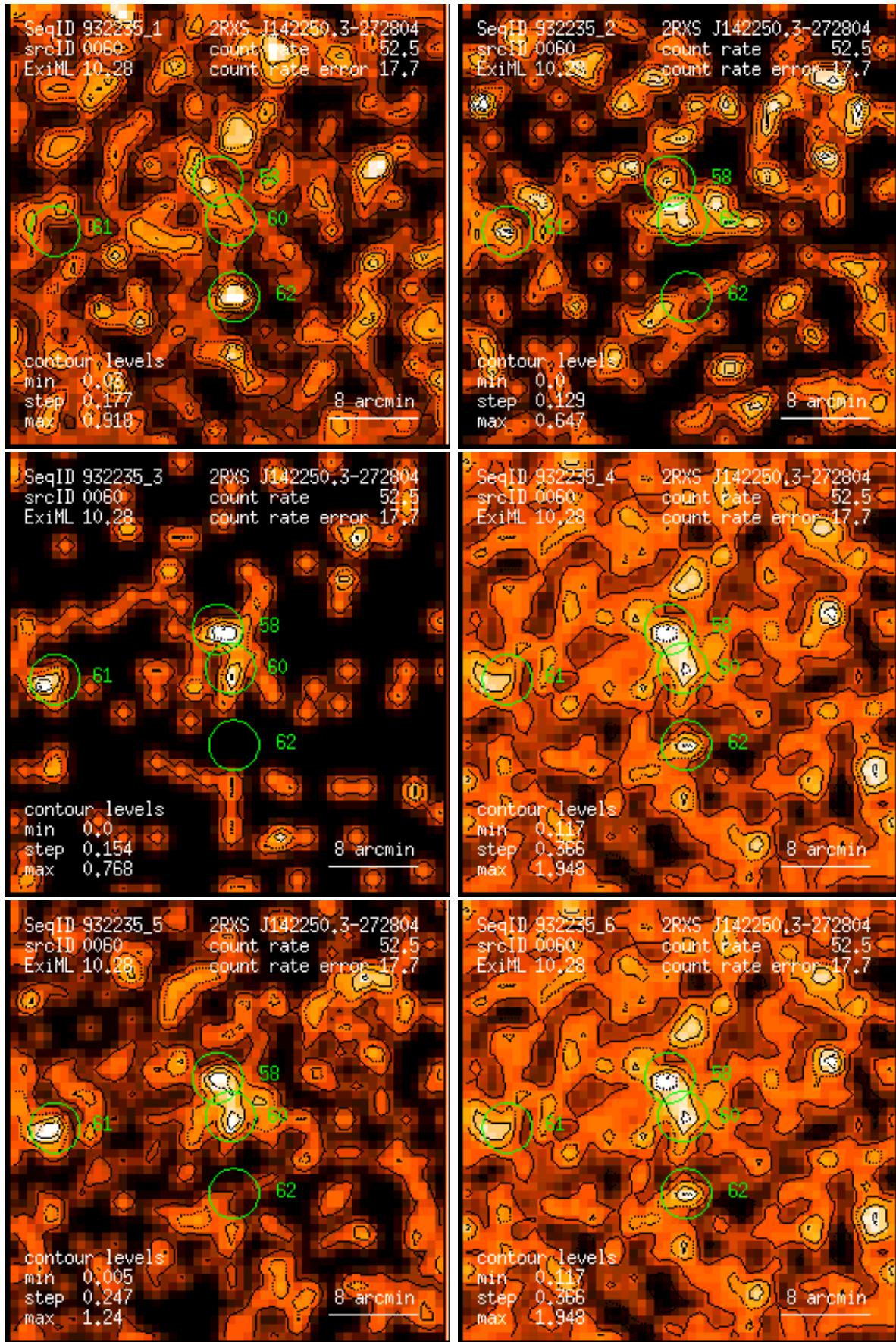
Figure 60: RASS 932235: detection 0060: band rate images, Gaussian filter: (1) PSPC channels 11 – 41, (2) 52 – 90, (3) 91 – 201, (4) 11 – 235, (5) 52 – 201, (6) 11 – 201. Broad band rates in counts/ks. Band rate contour levels in counts/ks/arcmin 2 .
