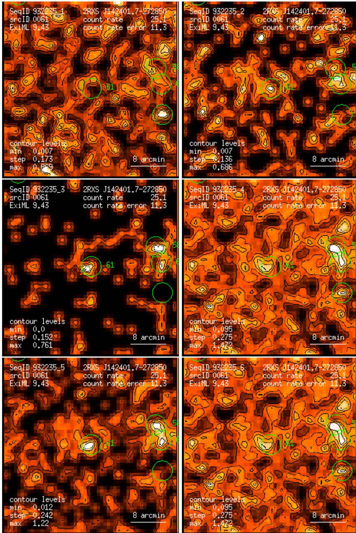
Figure 61: RASS 932235: detection 0061: band rate images, Gaussian filter: (1) PSPC channels 11 – 41, (2) 52 – 90, (3) 91 – 201, (4) 11 – 235, (5) 52 – 201, (6) 11 – 201. Broad band rates in counts/ks. Band rate contour levels in counts/ks/arcmin 2 .
