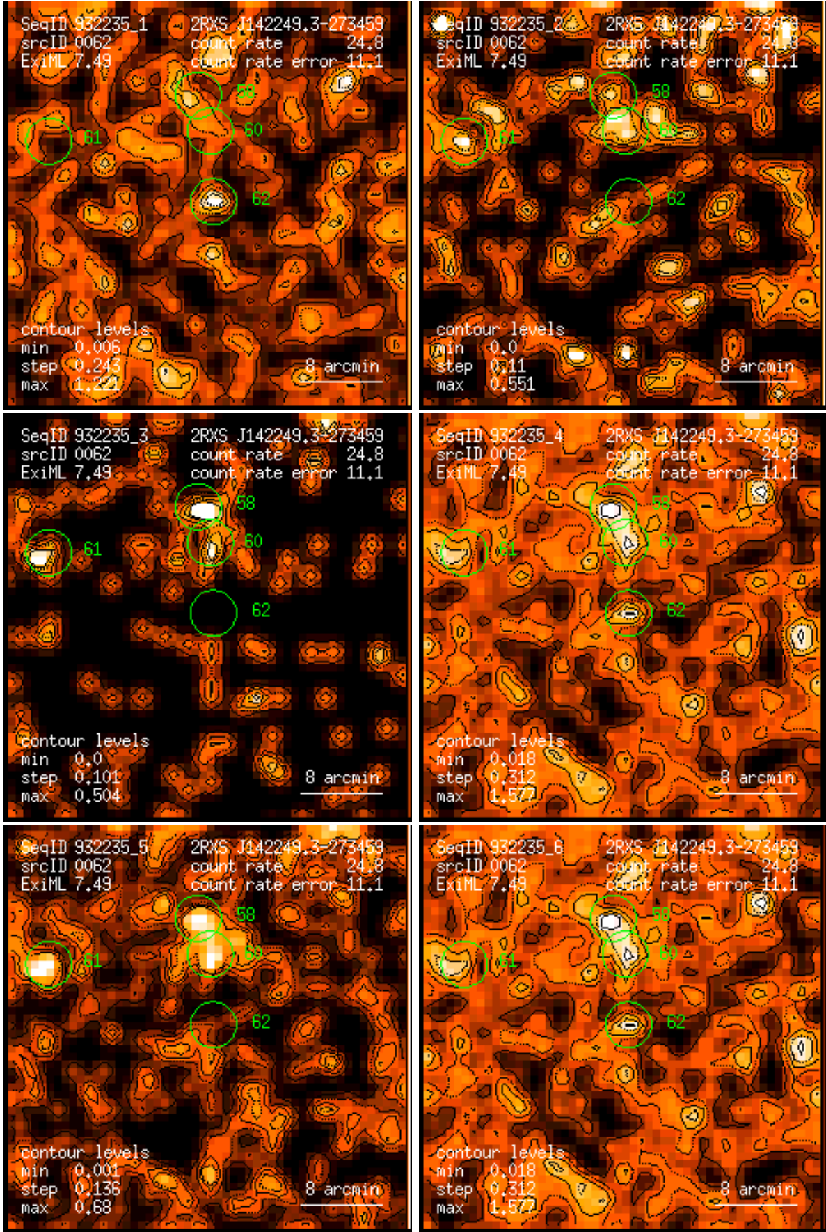
Figure 62: RASS 932235: detection 0062: band rate images, Gaussian filter: (1) PSPC channels 11 – 41, (2) 52 – 90, (3) 91 – 201, (4) 11 – 235, (5) 52 – 201, (6) 11 – 201. Broad band rates in counts/ks. Band rate contour levels in counts/ks/arcmin 2 .
