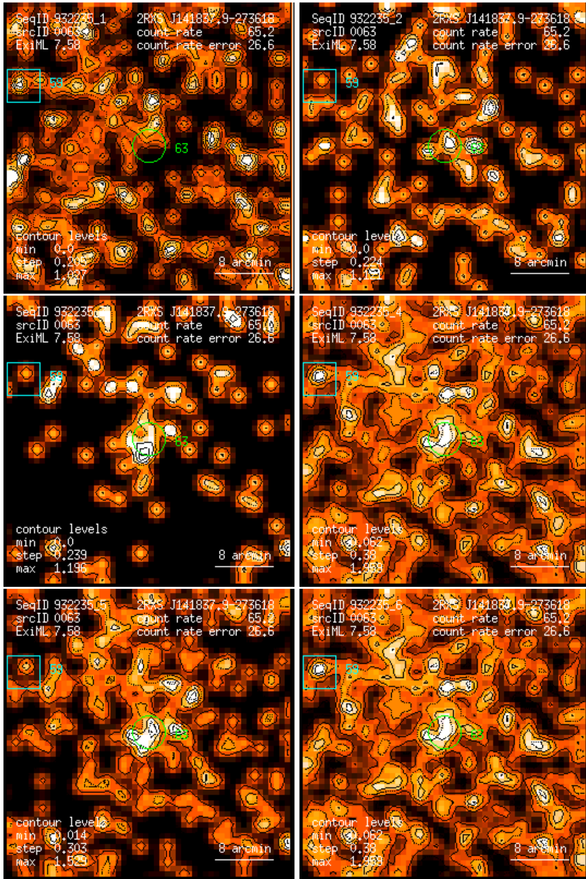
Figure 63: RASS 932235: detection 0063: band rate images, Gaussian filter: (1) PSPC channels 11 – 41, (2) 52 – 90, (3) 91 – 201, (4) 11 – 235, (5) 52 – 201, (6) 11 – 201. Broad band rates in counts/ks. Band rate contour levels in counts/ks/arcmin 2 .
