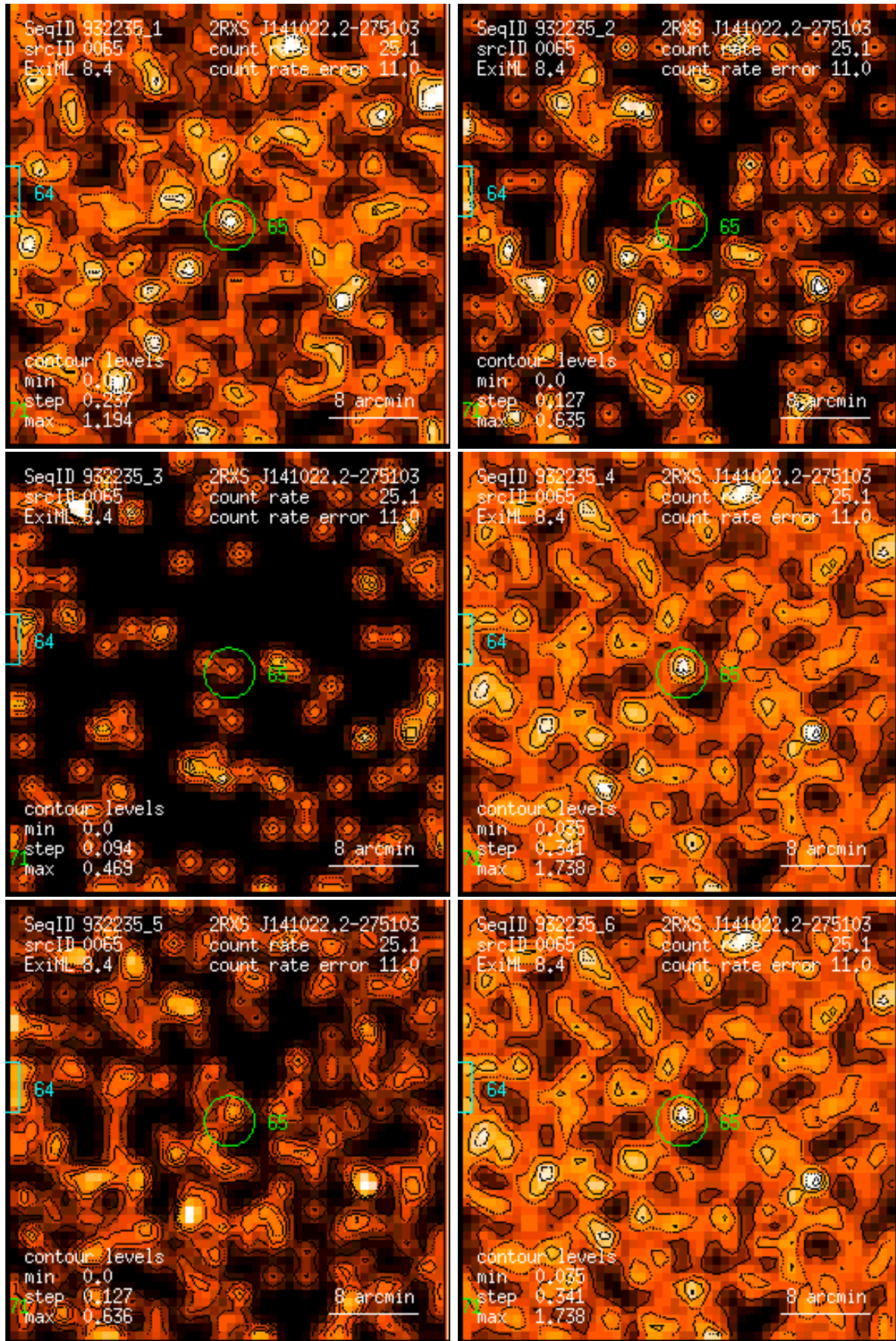
Figure 65: RASS 932235: detection 0065: band rate images, Gaussian filter: (1) PSPC channels 11 – 41, (2) 52 – 90, (3) 91 – 201, (4) 11 – 235, (5) 52 – 201, (6) 11 – 201. Broad band rates in counts/ks. Band rate contour levels in counts/ks/arcmin 2 .
