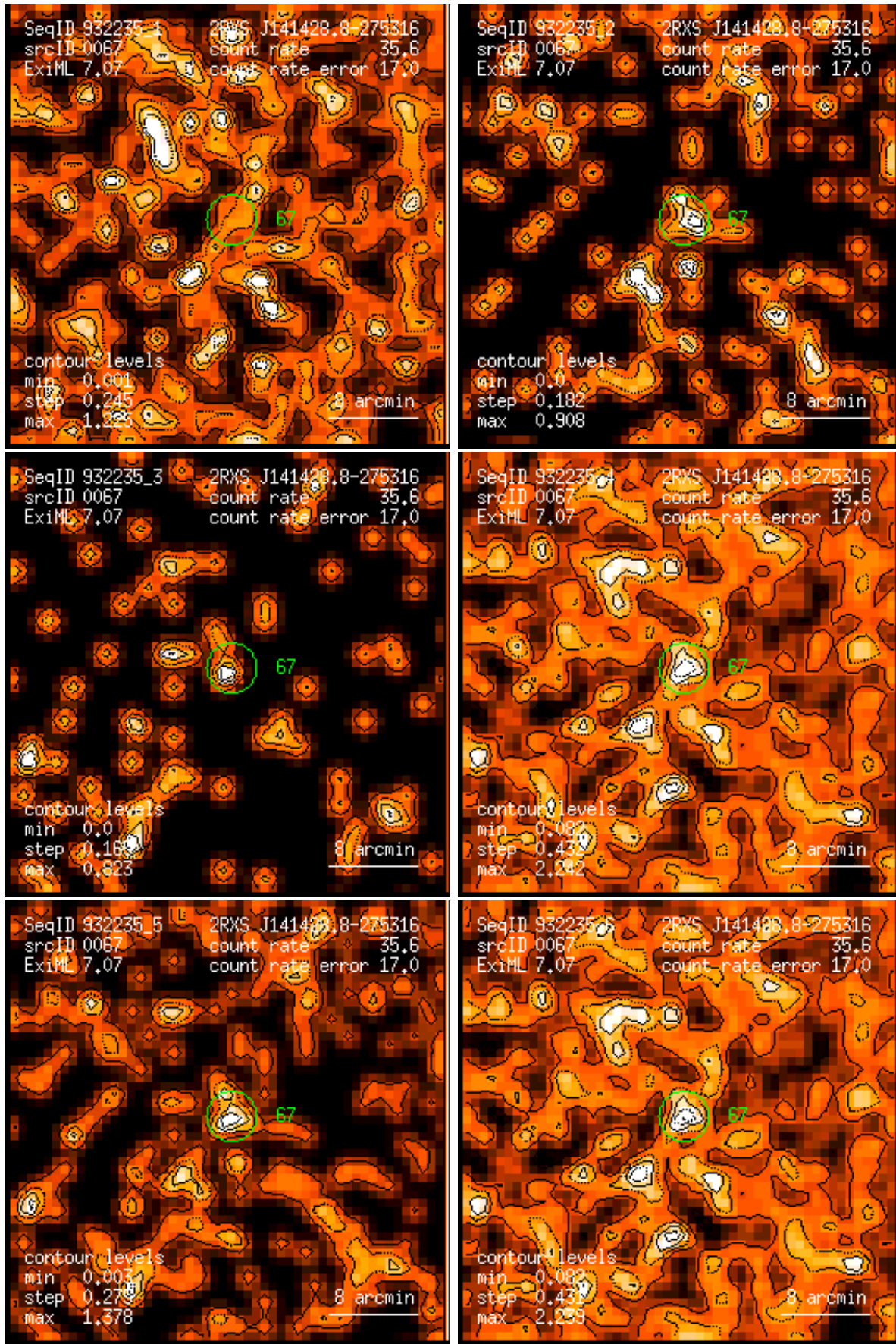
Figure 67: RASS 932235: detection 0067: band rate images, Gaussian filter: (1) PSPC channels 11 – 41, (2) 52 – 90, (3) 91 – 201, (4) 11 – 235, (5) 52 – 201, (6) 11 – 201. Broad band rates in counts/ks. Band rate contour levels in counts/ks/arcmin 2 .
