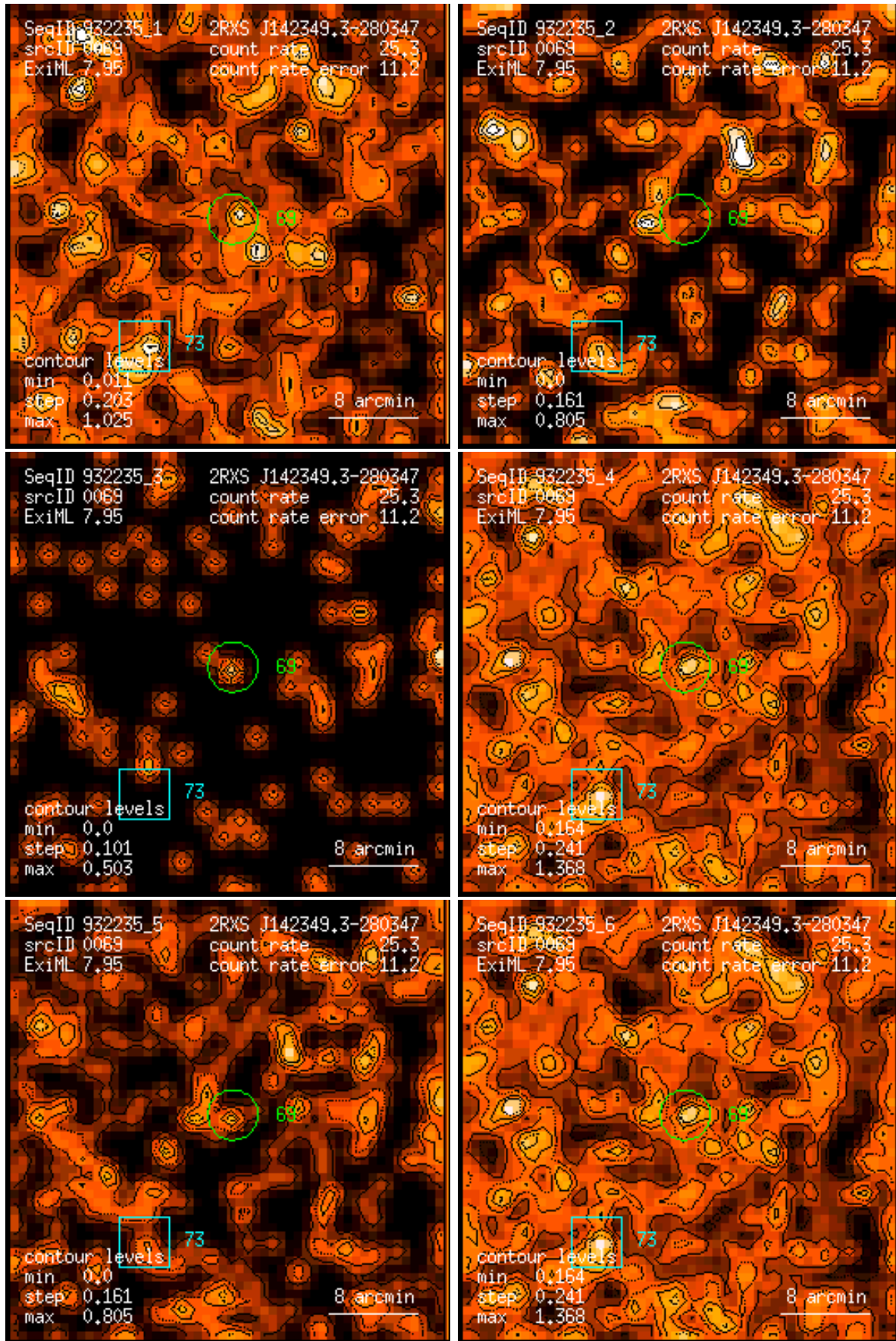
Figure 69: RASS 932235: detection 0069: band rate images, Gaussian filter: (1) PSPC channels 11 – 41, (2) 52 – 90, (3) 91 – 201, (4) 11 – 235, (5) 52 – 201, (6) 11 – 201. Broad band rates in counts/ks. Band rate contour levels in counts/ks/arcmin 2 .
