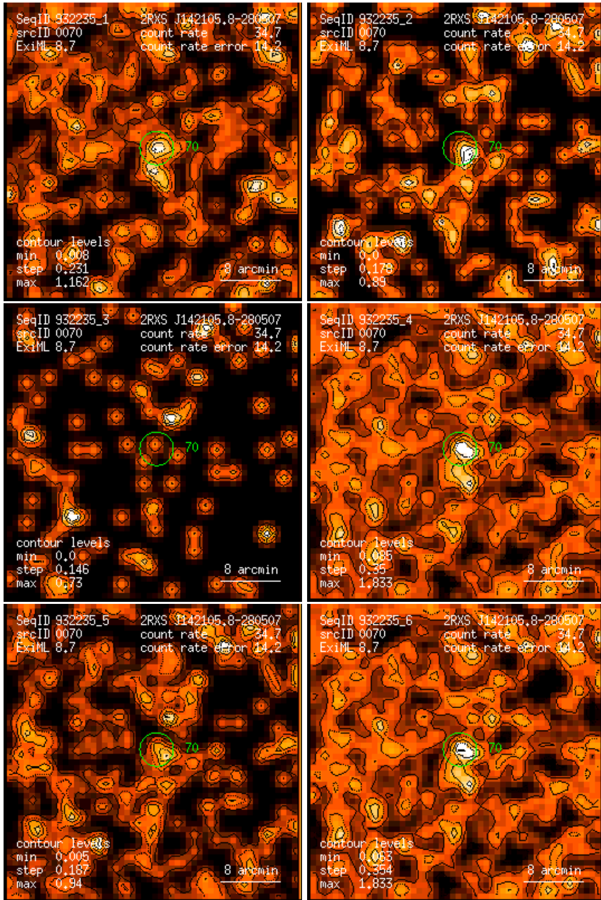
Figure 70: RASS 932235: detection 0070: band rate images, Gaussian filter: (1) PSPC channels 11 – 41, (2) 52 – 90, (3) 91 – 201, (4) 11 – 235, (5) 52 – 201, (6) 11 – 201. Broad band rates in counts/ks. Band rate contour levels in counts/ks/arcmin 2 .
