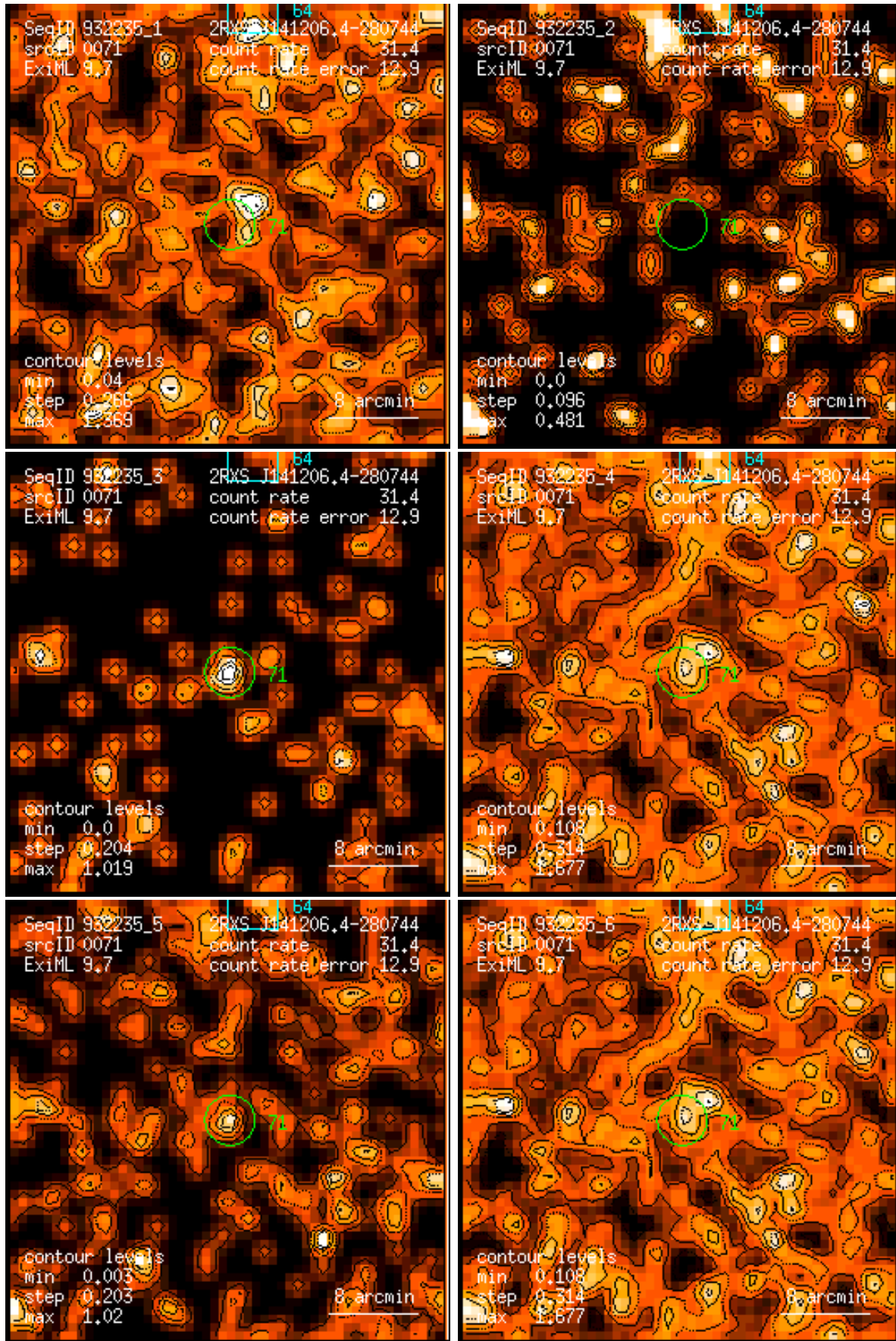
Figure 71: RASS 932235: detection 0071: band rate images, Gaussian filter: (1) PSPC channels 11 – 41, (2) 52 – 90, (3) 91 – 201, (4) 11 – 235, (5) 52 – 201, (6) 11 – 201. Broad band rates in counts/ks. Band rate contour levels in counts/ks/arcmin 2 .
