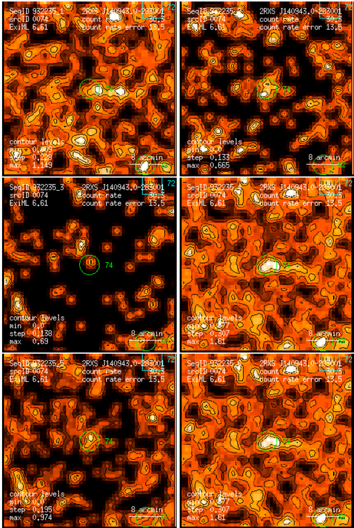
Figure 74: RASS 932235: detection 0074: band rate images, Gaussian filter: (1) PSPC channels 11 – 41, (2) 52 – 90, (3) 91 – 201, (4) 11 – 235, (5) 52 – 201, (6) 11 – 201. Broad band rates in counts/ks. Band rate contour levels in counts/ks/arcmin 2 .
