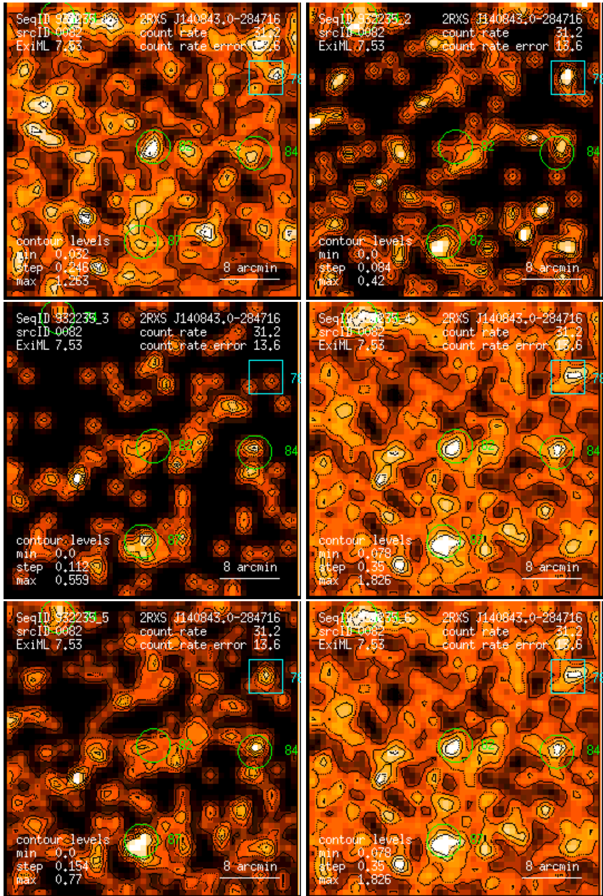
Figure 82: RASS 932235: detection 0082: band rate images, Gaussian filter: (1) PSPC channels 11 – 41, (2) 52 – 90, (3) 91 – 201, (4) 11 – 235, (5) 52 – 201, (6) 11 – 201. Broad band rates in counts/ks. Band rate contour levels in counts/ks/arcmin 2 .
