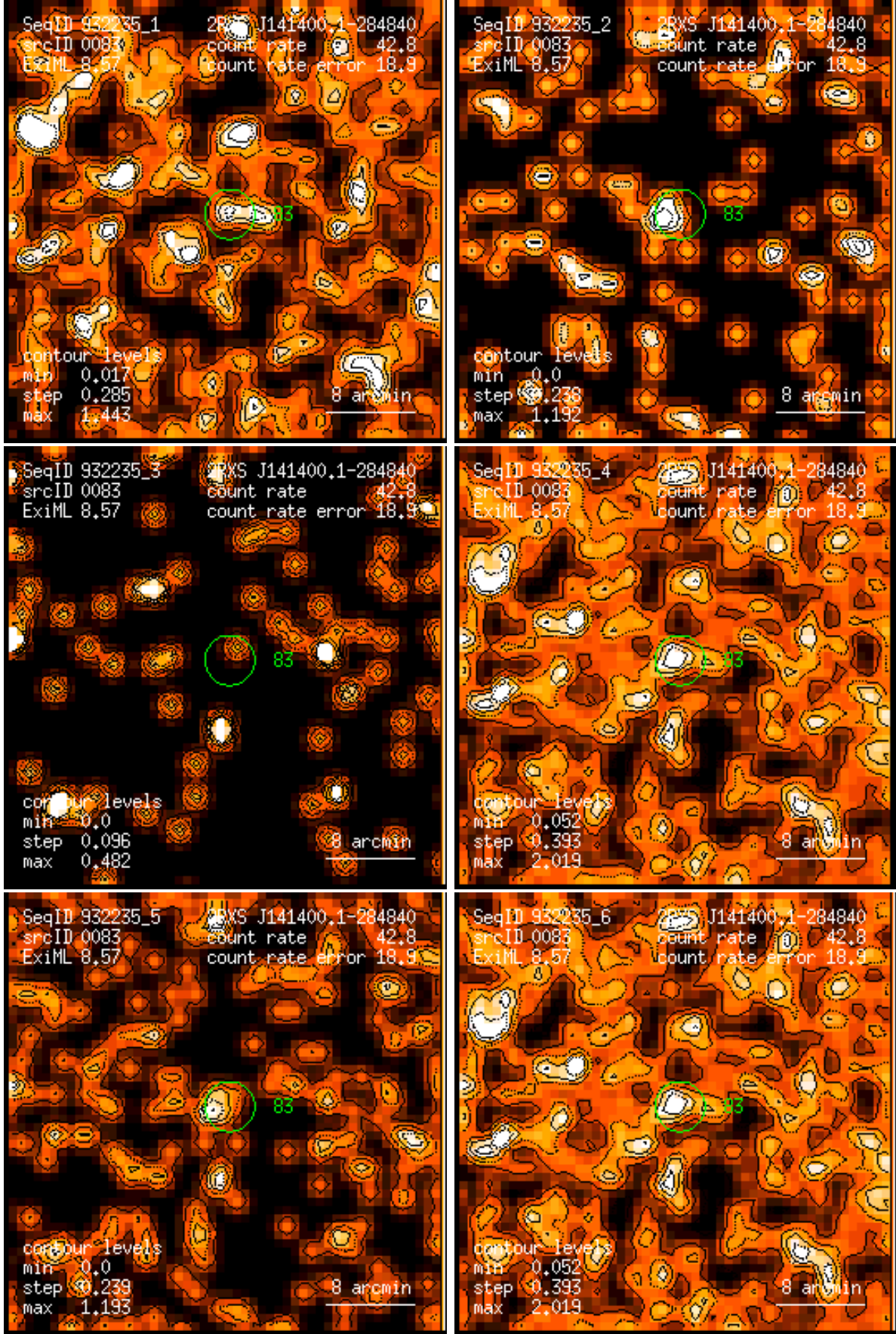
Figure 83: RASS 932235: detection 0083: band rate images, Gaussian filter: (1) PSPC channels 11 – 41, (2) 52 – 90, (3) 91 – 201, (4) 11 – 235, (5) 52 – 201, (6) 11 – 201. Broad band rates in counts/ks. Band rate contour levels in counts/ks/arcmin 2 .
