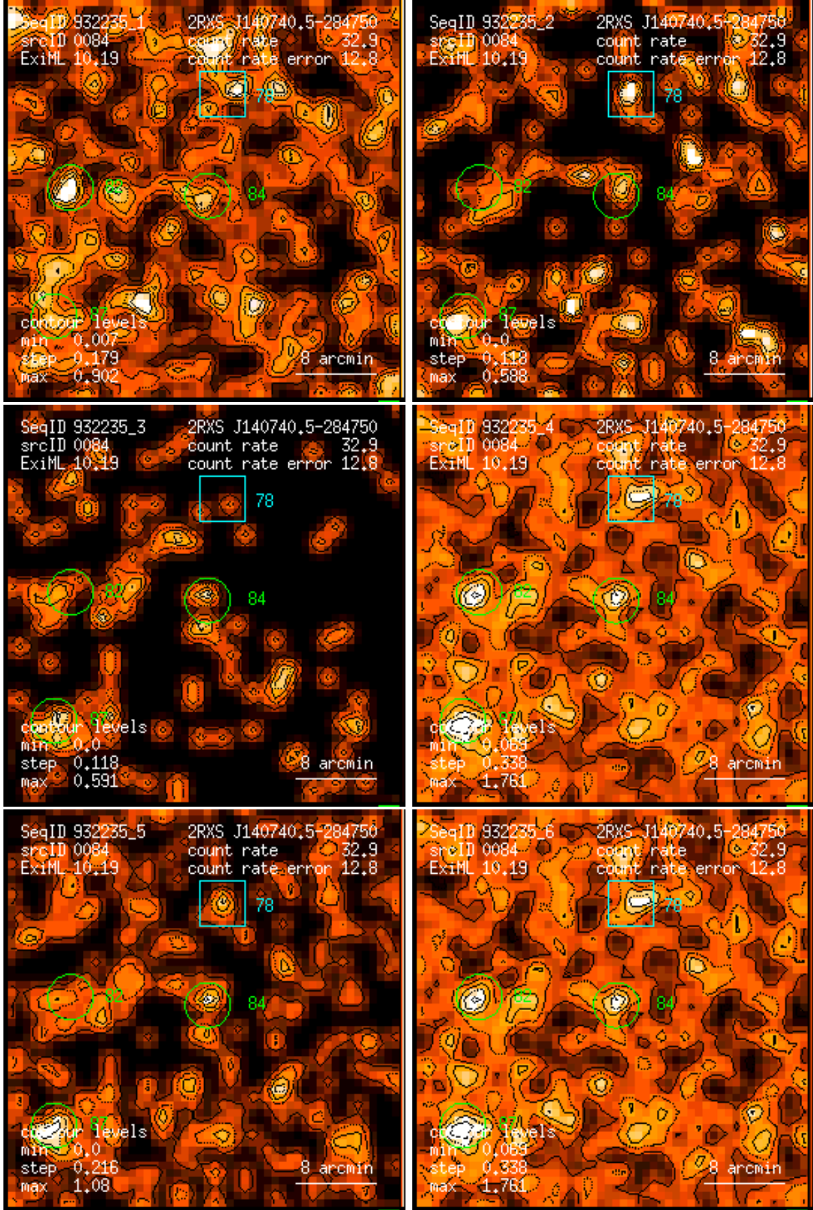
Figure 84: RASS 932235: detection 0084: band rate images, Gaussian filter: (1) PSPC channels 11 – 41, (2) 52 – 90, (3) 91 – 201, (4) 11 – 235, (5) 52 – 201, (6) 11 – 201. Broad band rates in counts/ks. Band rate contour levels in counts/ks/arcmin 2 .
