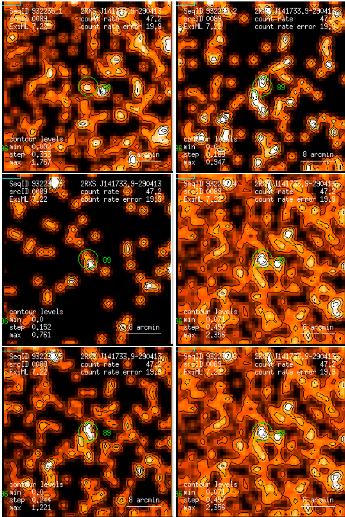
Figure 89: RASS 932235: detection 0089: band rate images, Gaussian filter: (1) PSPC channels 11 – 41, (2) 52 – 90, (3) 91 – 201, (4) 11 – 235, (5) 52 – 201, (6) 11 – 201. Broad band rates in counts/ks. Band rate contour levels in counts/ks/arcmin 2 .
