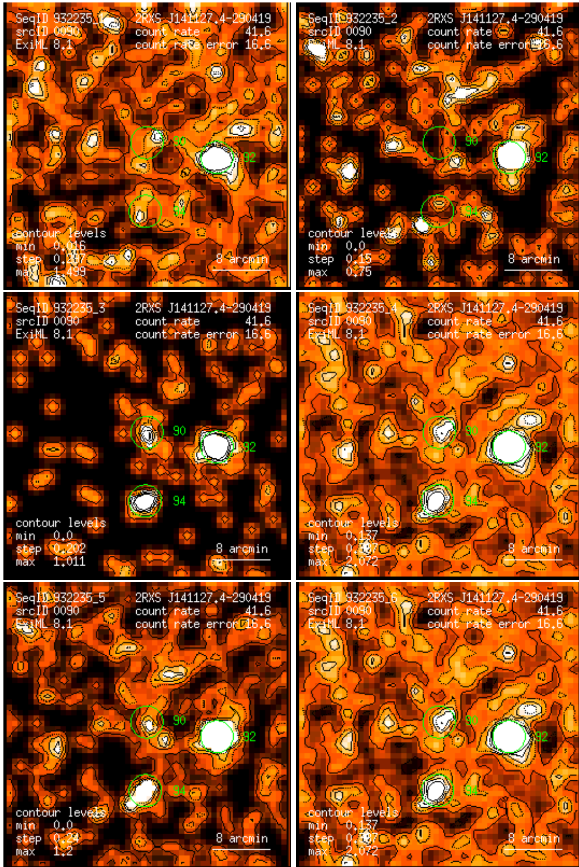
Figure 90: RASS 932235: detection 0090: band rate images, Gaussian filter: (1) PSPC channels 11 – 41, (2) 52 – 90, (3) 91 – 201, (4) 11 – 235, (5) 52 – 201, (6) 11 – 201. Broad band rates in counts/ks. Band rate contour levels in counts/ks/arcmin 2 .
