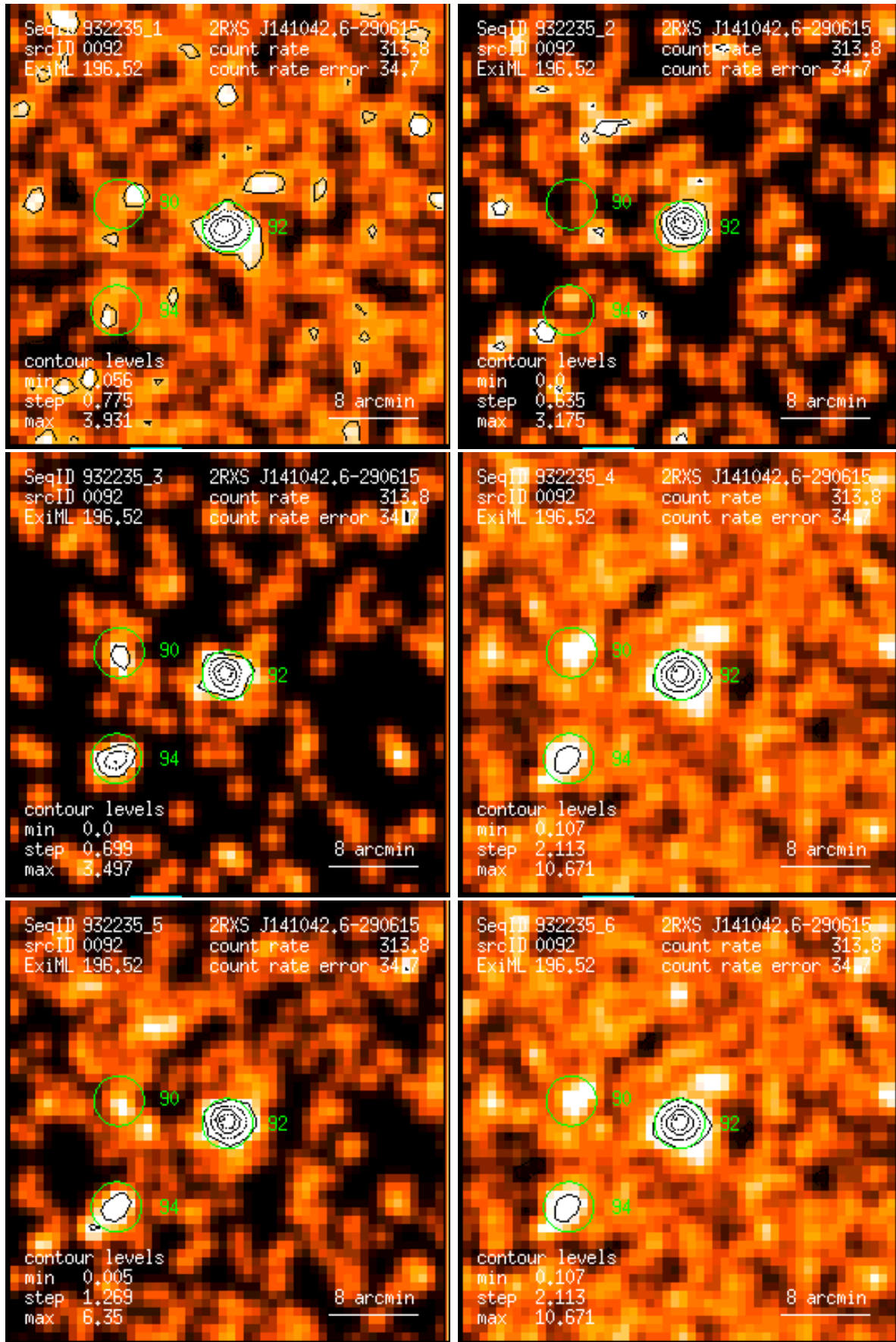
Figure 92: RASS 932235: detection 0092: band rate images, Gaussian filter: (1) PSPC channels 11 – 41, (2) 52 – 90, (3) 91 – 201, (4) 11 – 235, (5) 52 – 201, (6) 11 – 201. Broad band rates in counts/ks. Band rate contour levels in counts/ks/arcmin 2 .
