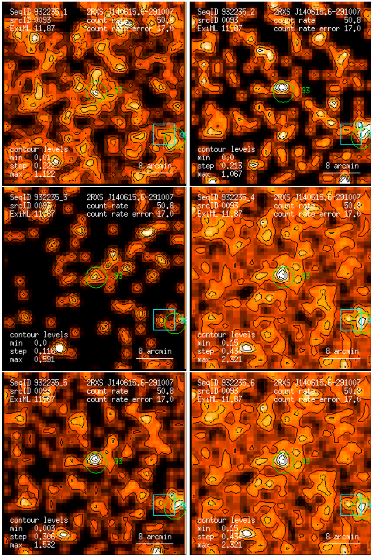
Figure 93: RASS 932235: detection 0093: band rate images, Gaussian filter: (1) PSPC channels 11 – 41, (2) 52 – 90, (3) 91 – 201, (4) 11 – 235, (5) 52 – 201, (6) 11 – 201. Broad band rates in counts/ks. Band rate contour levels in counts/ks/arcmin 2 .
