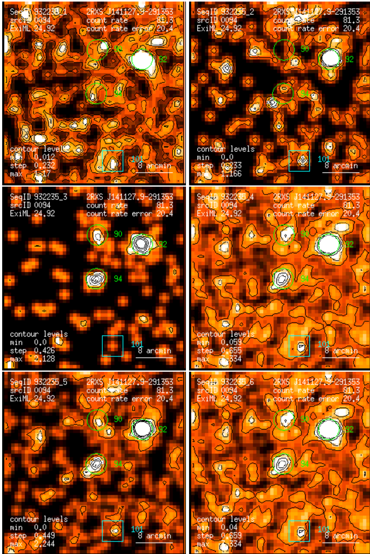
Figure 94: RASS 932235: detection 0094: band rate images, Gaussian filter: (1) PSPC channels 11 – 41, (2) 52 – 90, (3) 91 – 201, (4) 11 – 235, (5) 52 – 201, (6) 11 – 201. Broad band rates in counts/ks. Band rate contour levels in counts/ks/arcmin 2 .
