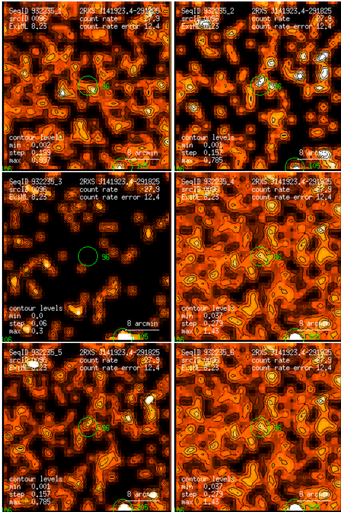
Figure 96: RASS 932235: detection 0096: band rate images, Gaussian filter: (1) PSPC channels 11 – 41, (2) 52 – 90, (3) 91 – 201, (4) 11 – 235, (5) 52 – 201, (6) 11 – 201. Broad band rates in counts/ks. Band rate contour levels in counts/ks/arcmin 2 .
