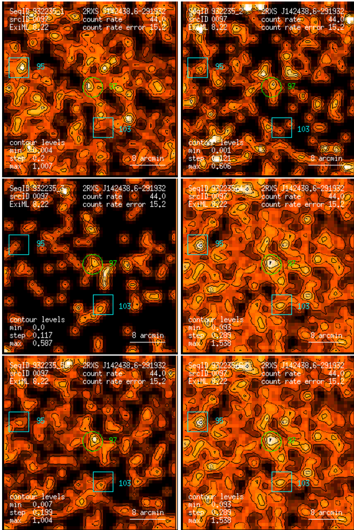
Figure 97: RASS 932235: detection 0097: band rate images, Gaussian filter: (1) PSPC channels 11 – 41, (2) 52 – 90, (3) 91 – 201, (4) 11 – 235, (5) 52 – 201, (6) 11 – 201. Broad band rates in counts/ks. Band rate contour levels in counts/ks/arcmin 2 .
