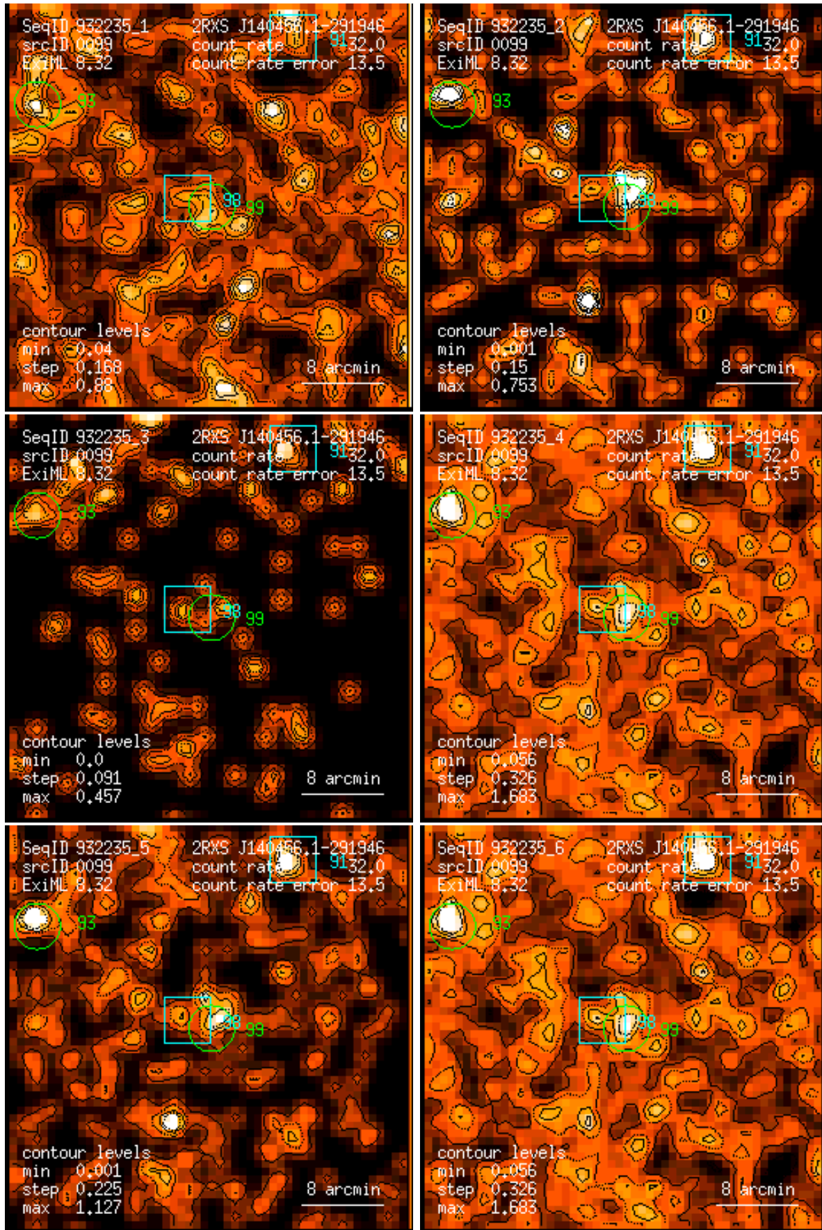
Figure 99: RASS 932235: detection 0099: band rate images, Gaussian filter: (1) PSPC channels 11 – 41, (2) 52 – 90, (3) 91 – 201, (4) 11 – 235, (5) 52 – 201, (6) 11 – 201. Broad band rates in counts/ks. Band rate contour levels in counts/ks/arcmin 2 .
