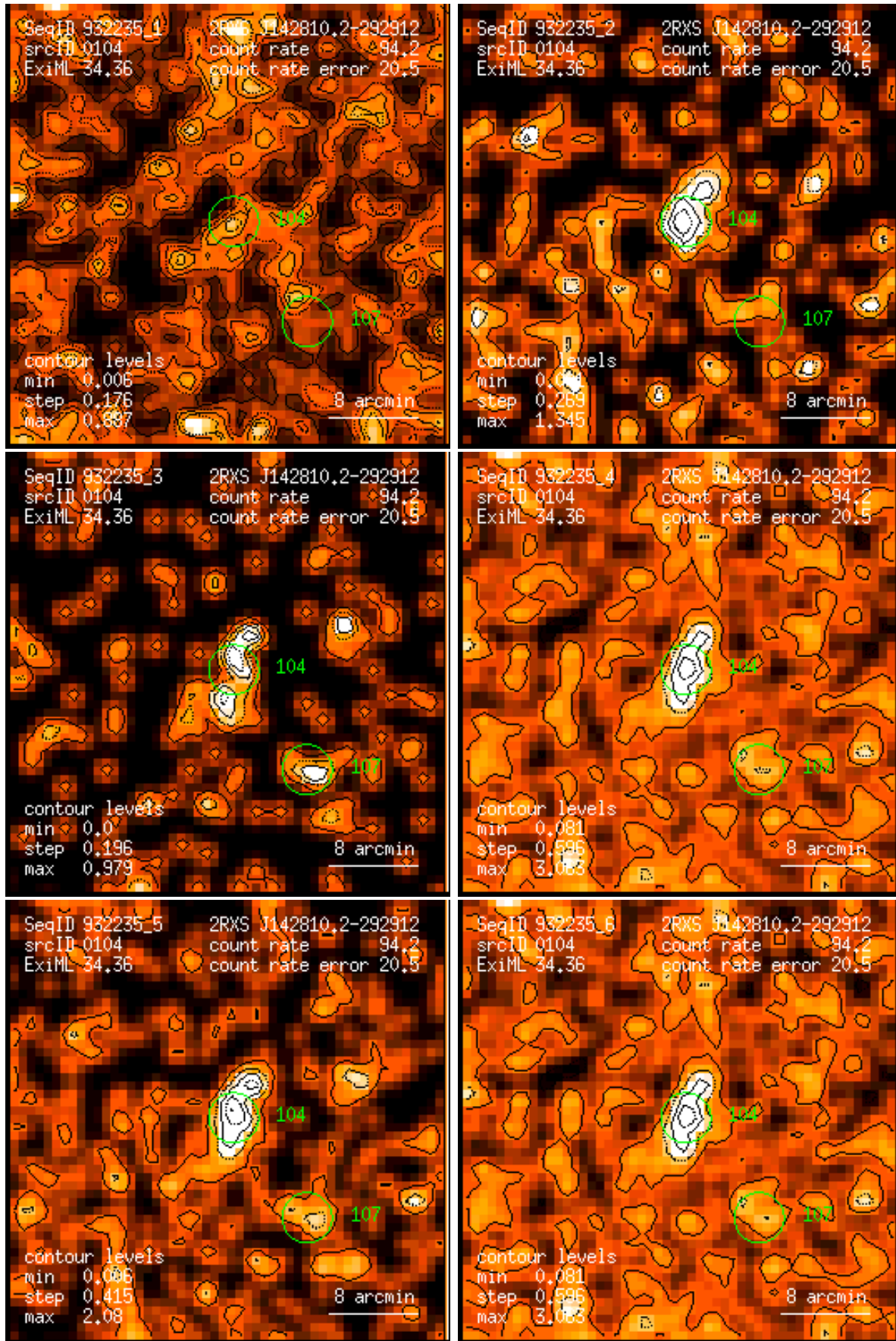
Figure 104: RASS 932235: detection 0104: band rate images, Gaussian filter: (1) PSPC channels 11 – 41, (2) 52 – 90, (3) 91 – 201, (4) 11 – 235, (5) 52 – 201, (6) 11 – 201. Broad band rates in counts/ks. Band rate contour levels in counts/ks/arcmin 2 .
