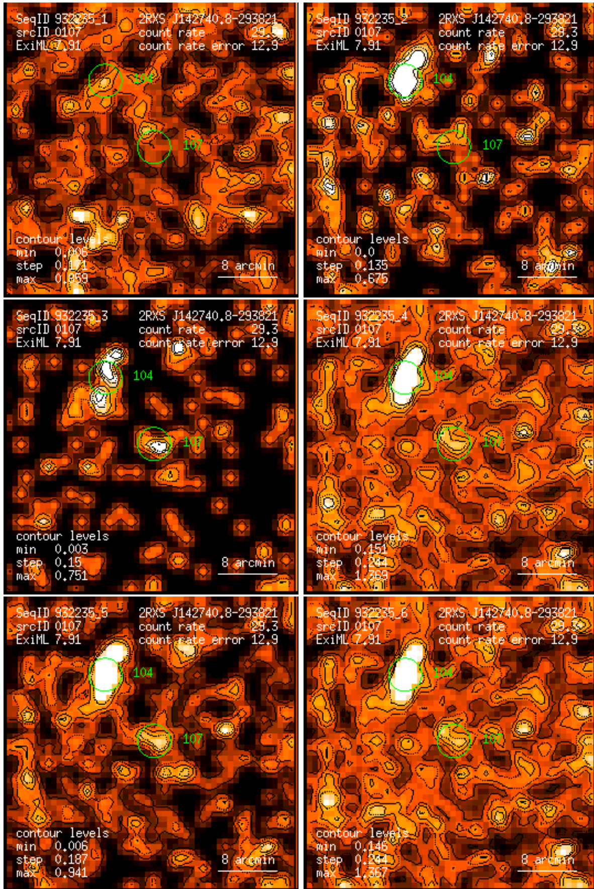
Figure 107: RASS 932235: detection 0107: band rate images, Gaussian filter: (1) PSPC channels 11 – 41, (2) 52 – 90, (3) 91 – 201, (4) 11 – 235, (5) 52 – 201, (6) 11 – 201. Broad band rates in counts/ks. Band rate contour levels in counts/ks/arcmin 2 .
