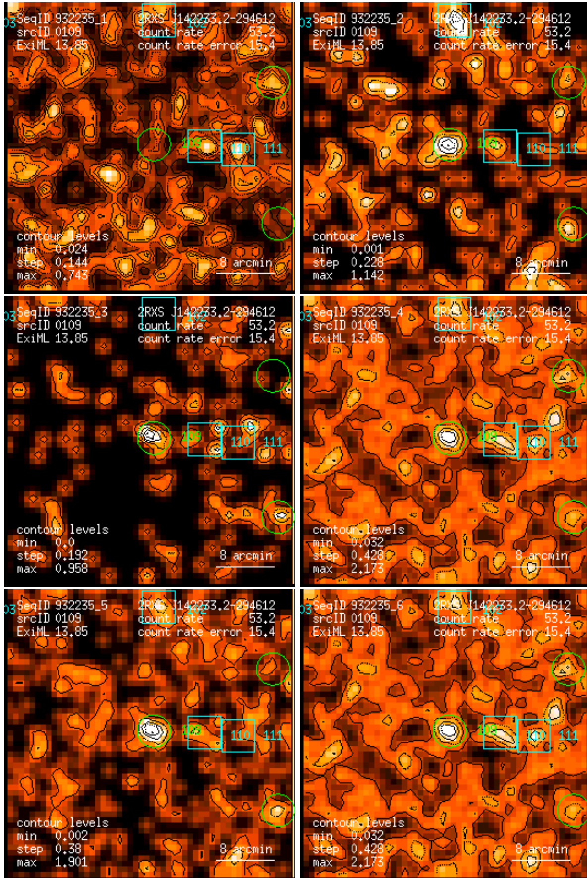
Figure 109: RASS 932235: detection 0109: band rate images, Gaussian filter: (1) PSPC channels 11 – 41, (2) 52 – 90, (3) 91 – 201, (4) 11 – 235, (5) 52 – 201, (6) 11 – 201. Broad band rates in counts/ks. Band rate contour levels in counts/ks/arcmin 2 .
