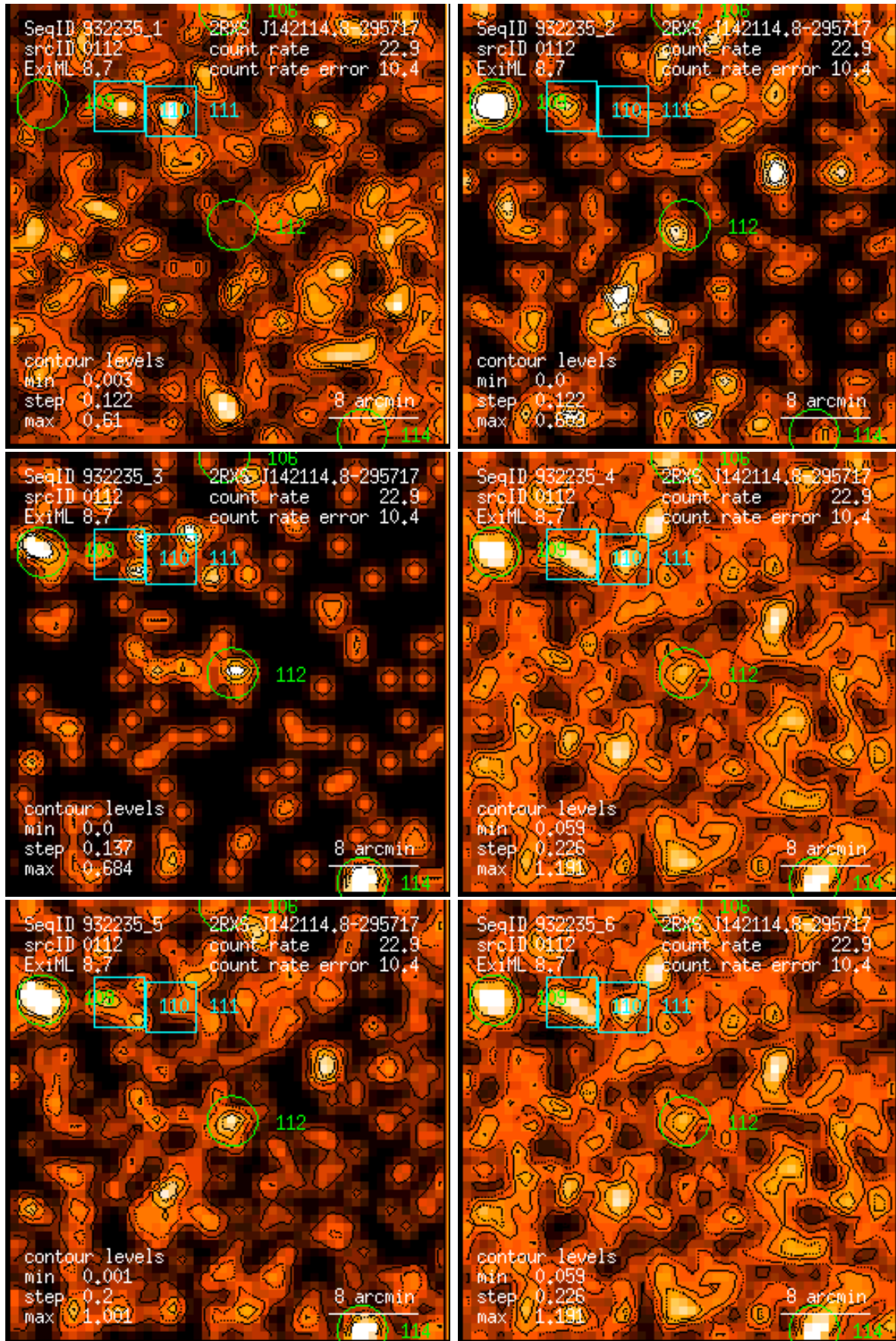
Figure 112: RASS 932235: detection 0112: band rate images, Gaussian filter: (1) PSPC channels 11 – 41, (2) 52 – 90, (3) 91 – 201, (4) 11 – 235, (5) 52 – 201, (6) 11 – 201. Broad band rates in counts/ks. Band rate contour levels in counts/ks/arcmin 2 .
