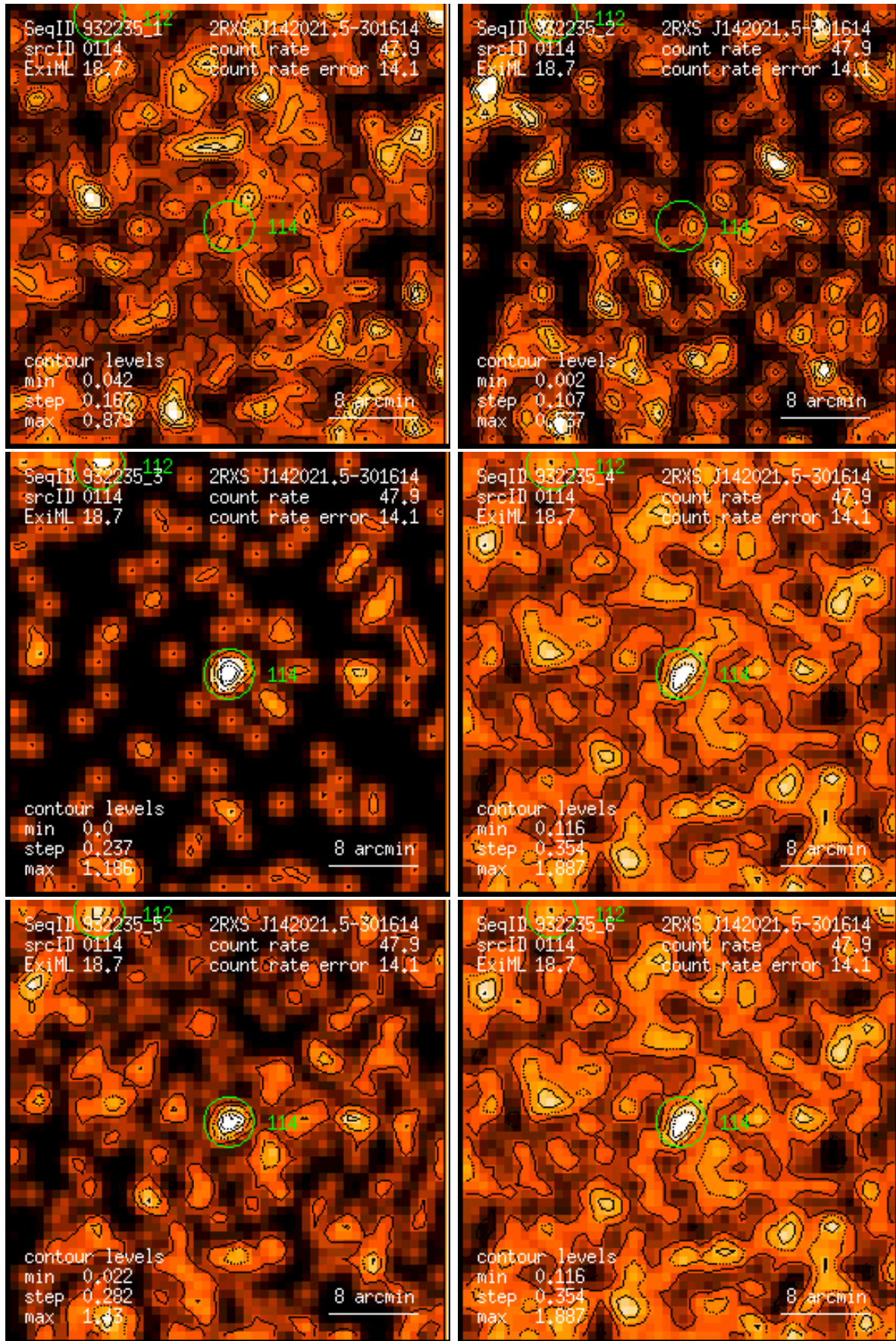
Figure 114: RASS 932235: detection 0114: band rate images, Gaussian filter: (1) PSPC channels 11 – 41, (2) 52 – 90, (3) 91 – 201, (4) 11 – 235, (5) 52 – 201, (6) 11 – 201. Broad band rates in counts/ks. Band rate contour levels in counts/ks/arcmin 2 .
