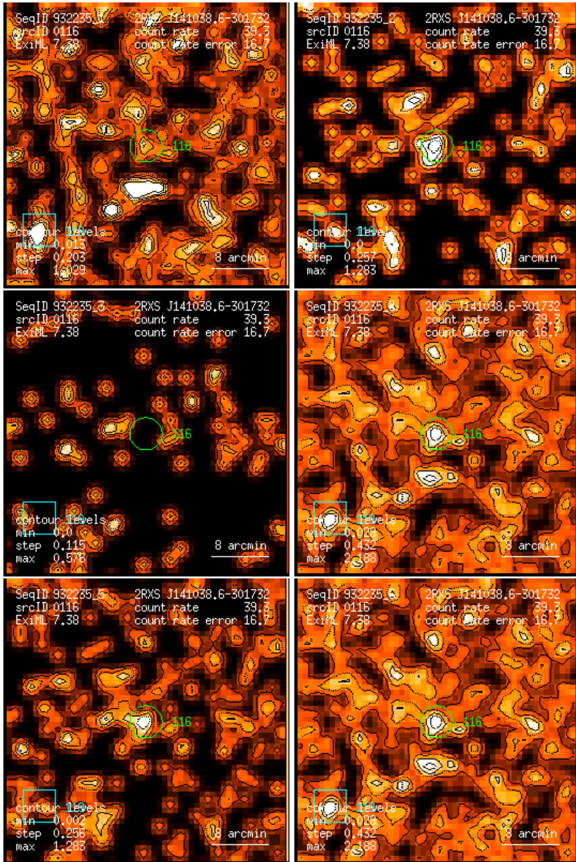
Figure 116: RASS 932235: detection 0116: band rate images, Gaussian filter: (1) PSPC channels 11 – 41, (2) 52 – 90, (3) 91 – 201, (4) 11 – 235, (5) 52 – 201, (6) 11 – 201. Broad band rates in counts/ks. Band rate contour levels in counts/ks/arcmin 2 .
