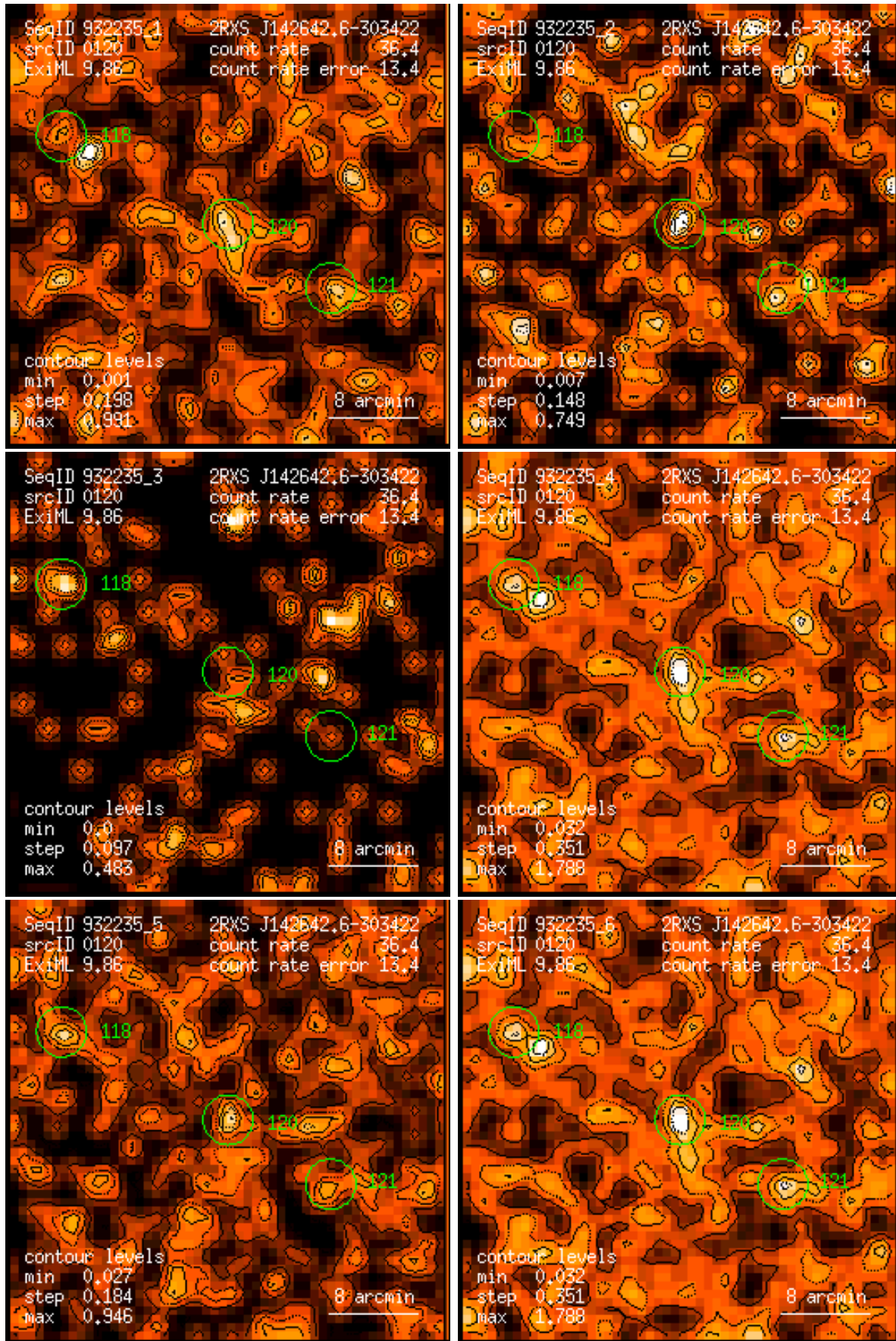
Figure 120: RASS 932235: detection 0120: band rate images, Gaussian filter: (1) PSPC channels 11 – 41, (2) 52 – 90, (3) 91 – 201, (4) 11 – 235, (5) 52 – 201, (6) 11 – 201. Broad band rates in counts/ks. Band rate contour levels in counts/ks/arcmin 2 .
