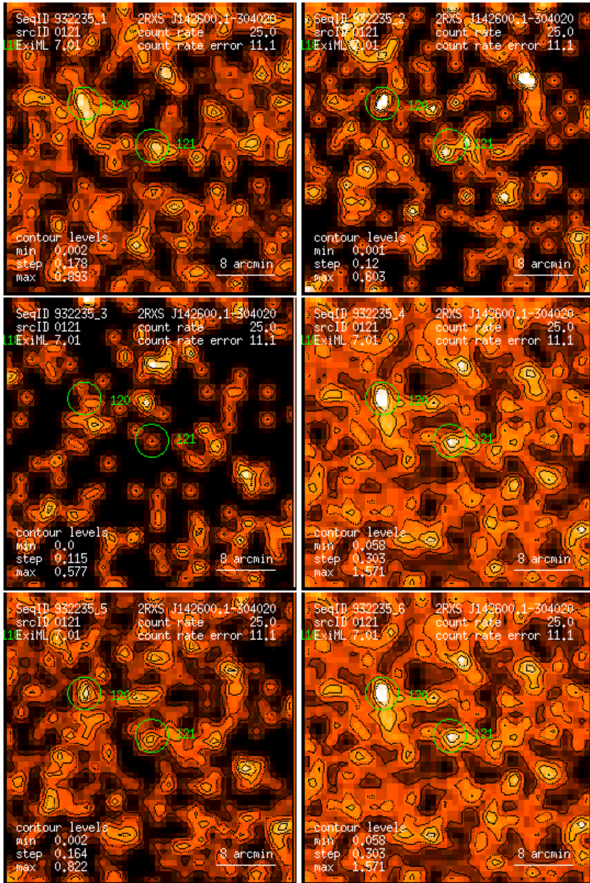
Figure 121: RASS 932235: detection 0121: band rate images, Gaussian filter: (1) PSPC channels 11 – 41, (2) 52 – 90, (3) 91 – 201, (4) 11 – 235, (5) 52 – 201, (6) 11 – 201. Broad band rates in counts/ks. Band rate contour levels in counts/ks/arcmin 2 .
