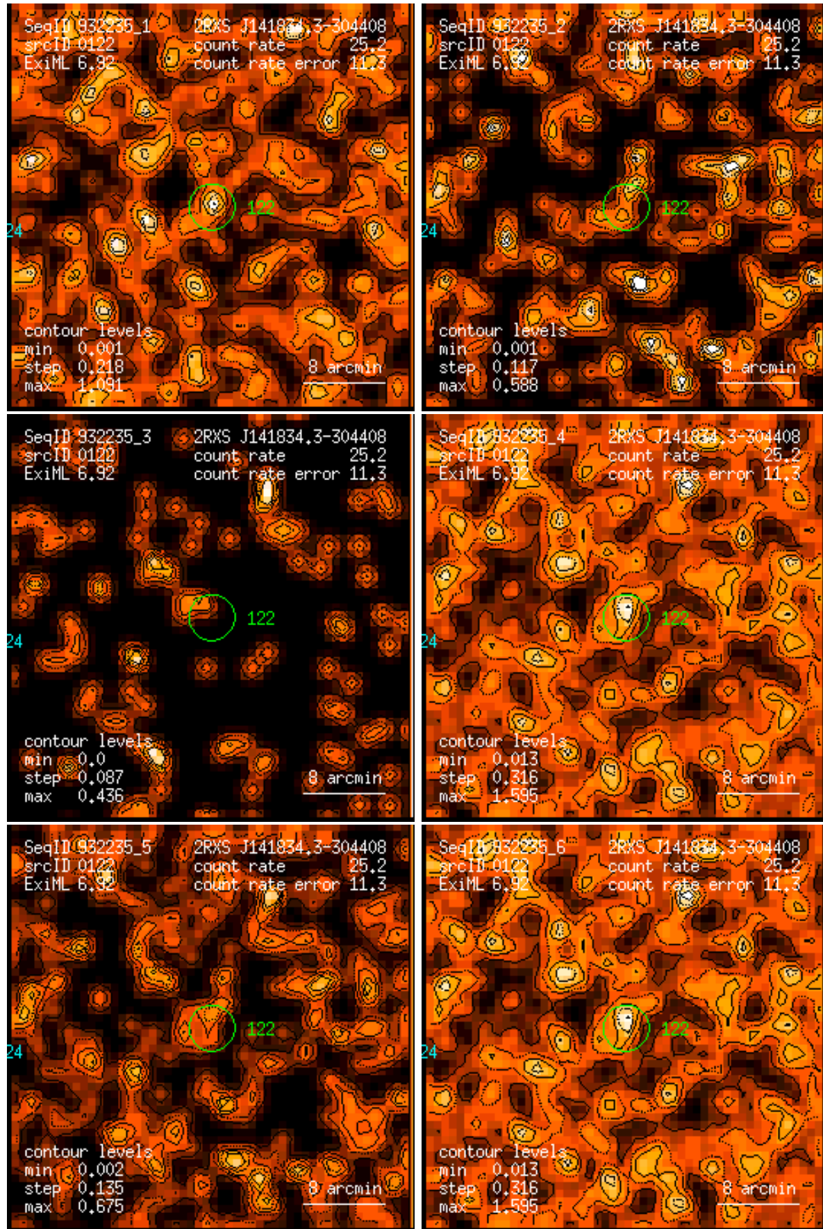
Figure 122: RASS 932235: detection 0122: band rate images, Gaussian filter: (1) PSPC channels 11 – 41, (2) 52 – 90, (3) 91 – 201, (4) 11 – 235, (5) 52 – 201, (6) 11 – 201. Broad band rates in counts/ks. Band rate contour levels in counts/ks/arcmin 2 .
