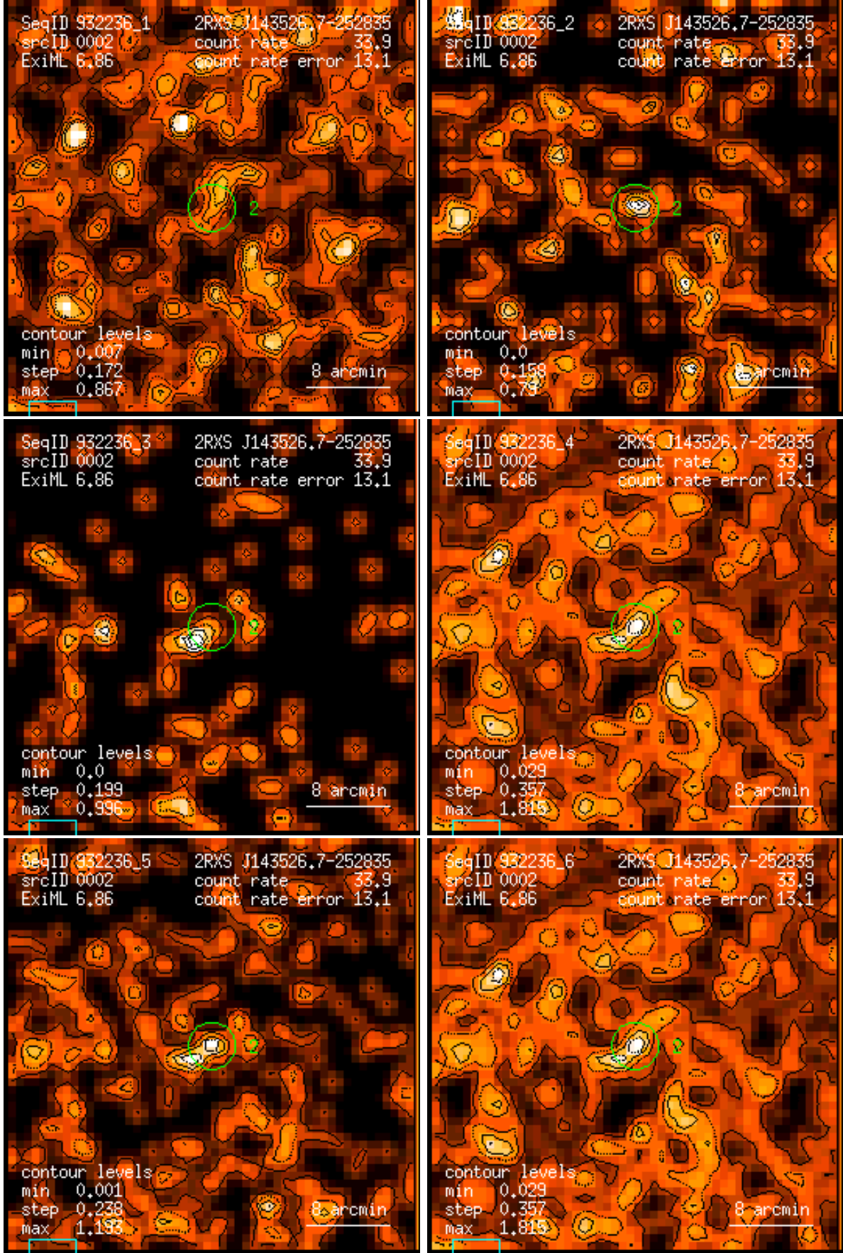
Figure 2: RASS 932236: detection 0002: band rate images, Gaussian filter: (1) PSPC channels 11 – 41, (2) 52 – 90, (3) 91 – 201, (4) 11 – 235, (5) 52 – 201, (6) 11 – 201. Broad band rates in counts/ks. Band rate contour levels in counts/ks/arcmin 2 .
