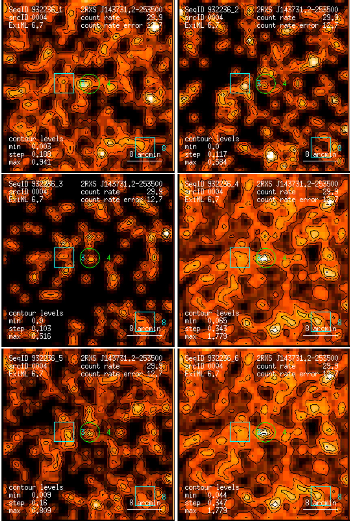
Figure 4: RASS 932236: detection 0004: band rate images, Gaussian filter: (1) PSPC channels 11 – 41, (2) 52 – 90, (3) 91 – 201, (4) 11 – 235, (5) 52 – 201, (6) 11 – 201. Broad band rates in counts/ks. Band rate contour levels in counts/ks/arcmin 2 .
